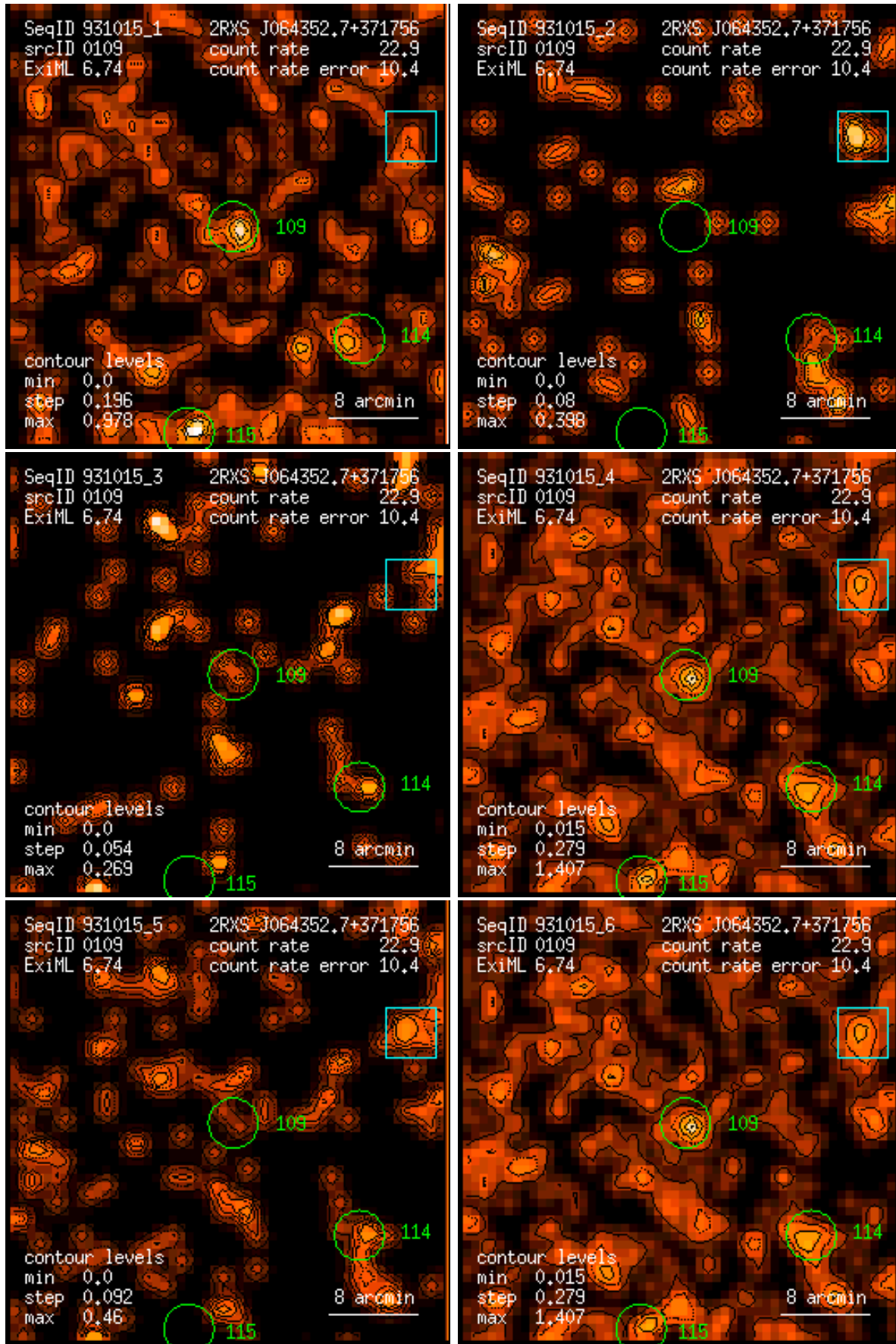
Figure 109: RASS 931015: detection 0109: band rate images, Gaussian filter: (1) PSPC channels 11 – 41, (2) 52 – 90, (3) 91 – 201, (4) 11 – 235, (5) 52 – 201, (6) 11 – 201. Broad band rates in counts/ks. Band rate contour levels in counts/ks/arcmin 2 .
