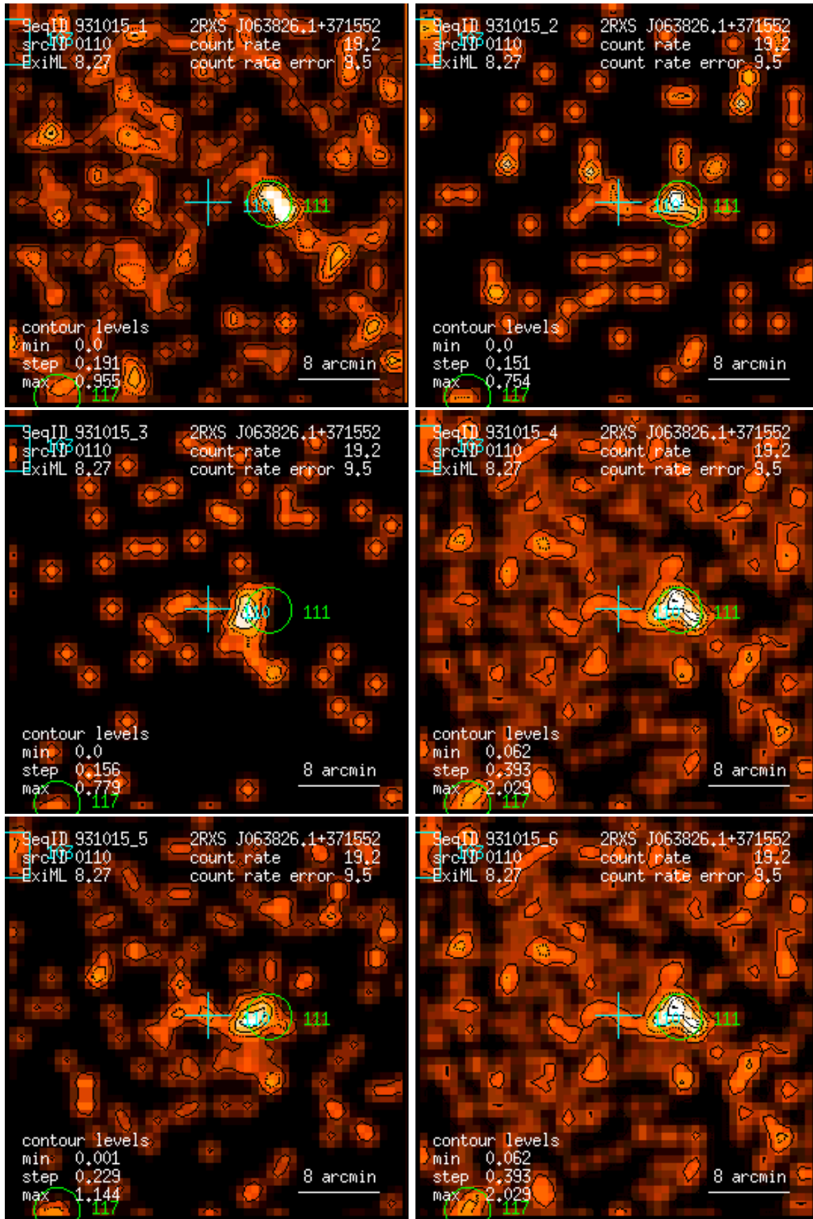
Figure 110: RASS 931015: detection 0110: band rate images, Gaussian filter: (1) PSPC channels 11 – 41, (2) 52 – 90, (3) 91 – 201, (4) 11 – 235, (5) 52 – 201, (6) 11 – 201. Broad band rates in counts/ks. Band rate contour levels in counts/ks/arcmin 2 .
