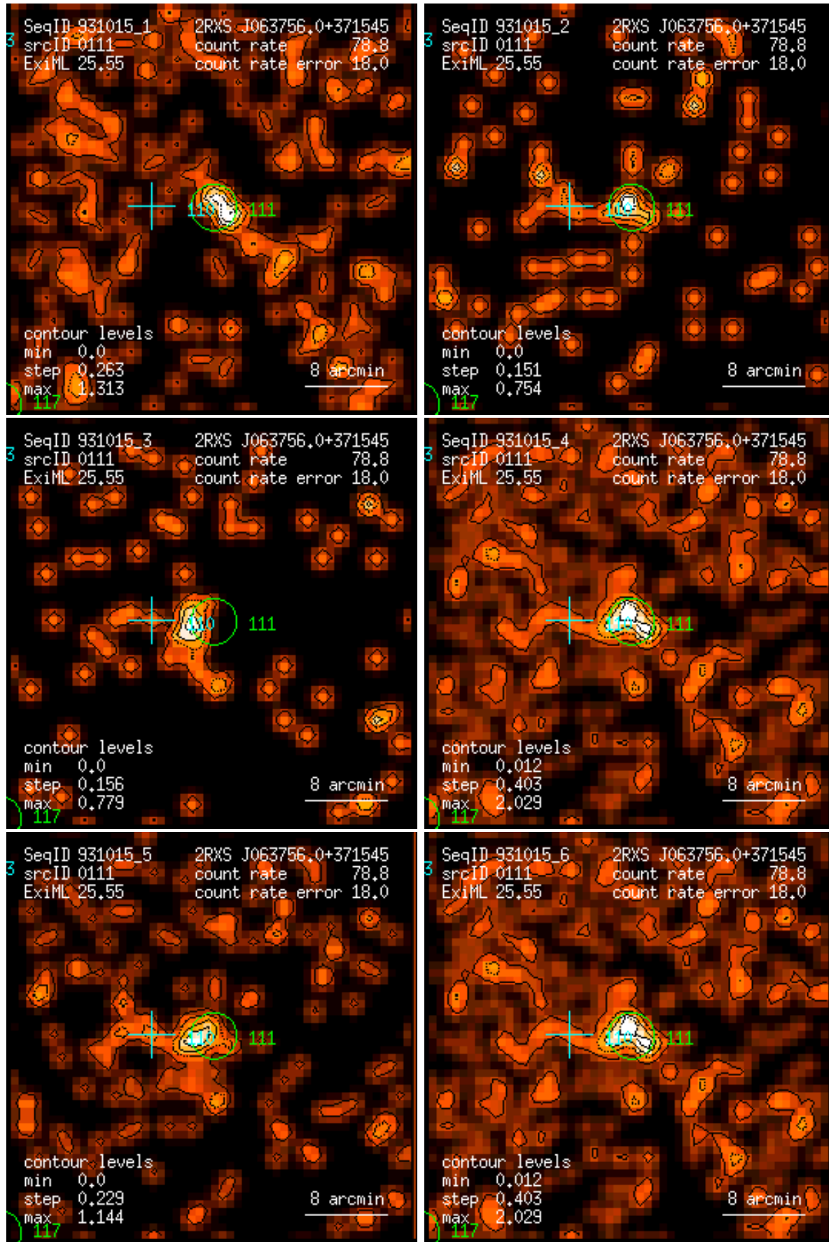
Figure 111: RASS 931015: detection 0111: band rate images, Gaussian filter: (1) PSPC channels 11 – 41, (2) 52 – 90, (3) 91 – 201, (4) 11 – 235, (5) 52 – 201, (6) 11 – 201. Broad band rates in counts/ks. Band rate contour levels in counts/ks/arcmin 2 .
