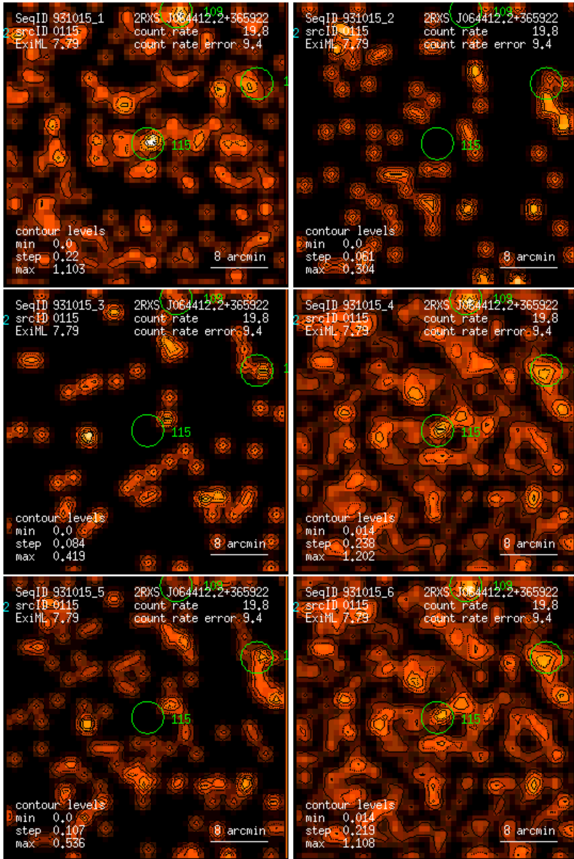
Figure 115: RASS 931015: detection 0115: band rate images, Gaussian filter: (1) PSPC channels 11 – 41, (2) 52 – 90, (3) 91 – 201, (4) 11 – 235, (5) 52 – 201, (6) 11 – 201. Broad band rates in counts/ks. Band rate contour levels in counts/ks/arcmin 2 .
