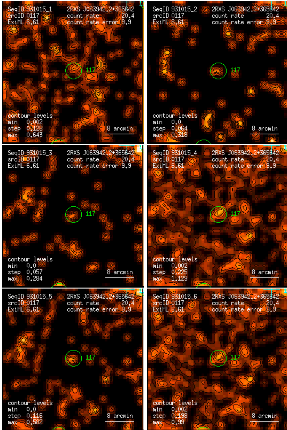
Figure 117: RASS 931015: detection 0117: band rate images, Gaussian filter: (1) PSPC channels 11 – 41, (2) 52 – 90, (3) 91 – 201, (4) 11 – 235, (5) 52 – 201, (6) 11 – 201. Broad band rates in counts/ks. Band rate contour levels in counts/ks/arcmin 2 .
