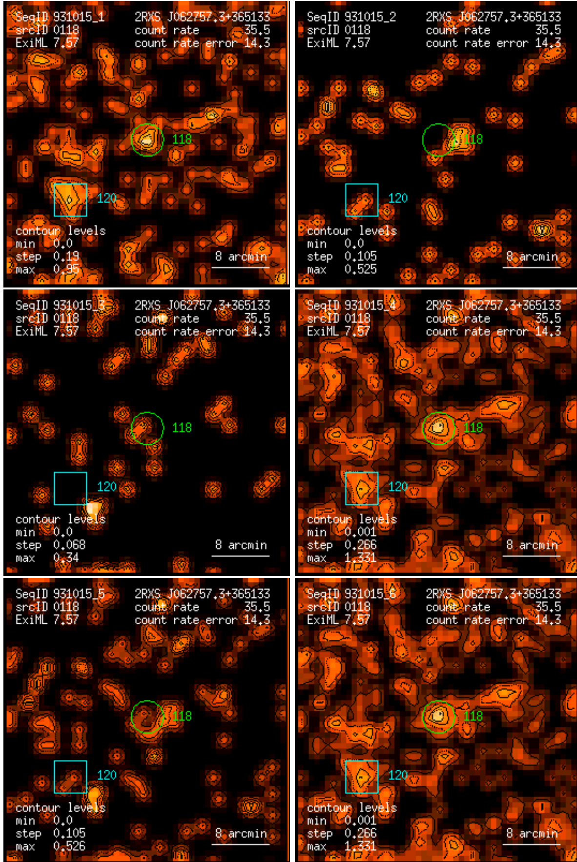
Figure 118: RASS 931015: detection 0118: band rate images, Gaussian filter: (1) PSPC channels 11 – 41, (2) 52 – 90, (3) 91 – 201, (4) 11 – 235, (5) 52 – 201, (6) 11 – 201. Broad band rates in counts/ks. Band rate contour levels in counts/ks/arcmin 2 .
