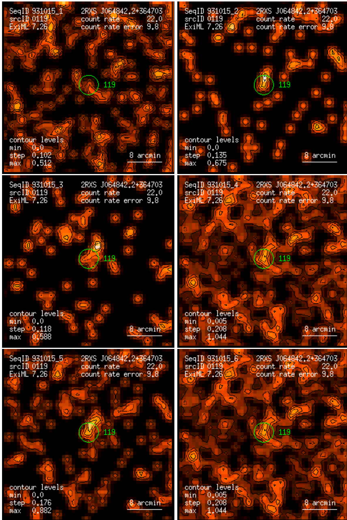
Figure 119: RASS 931015: detection 0119: band rate images, Gaussian filter: (1) PSPC channels 11 – 41, (2) 52 – 90, (3) 91 – 201, (4) 11 – 235, (5) 52 – 201, (6) 11 – 201. Broad band rates in counts/ks. Band rate contour levels in counts/ks/arcmin 2 .
