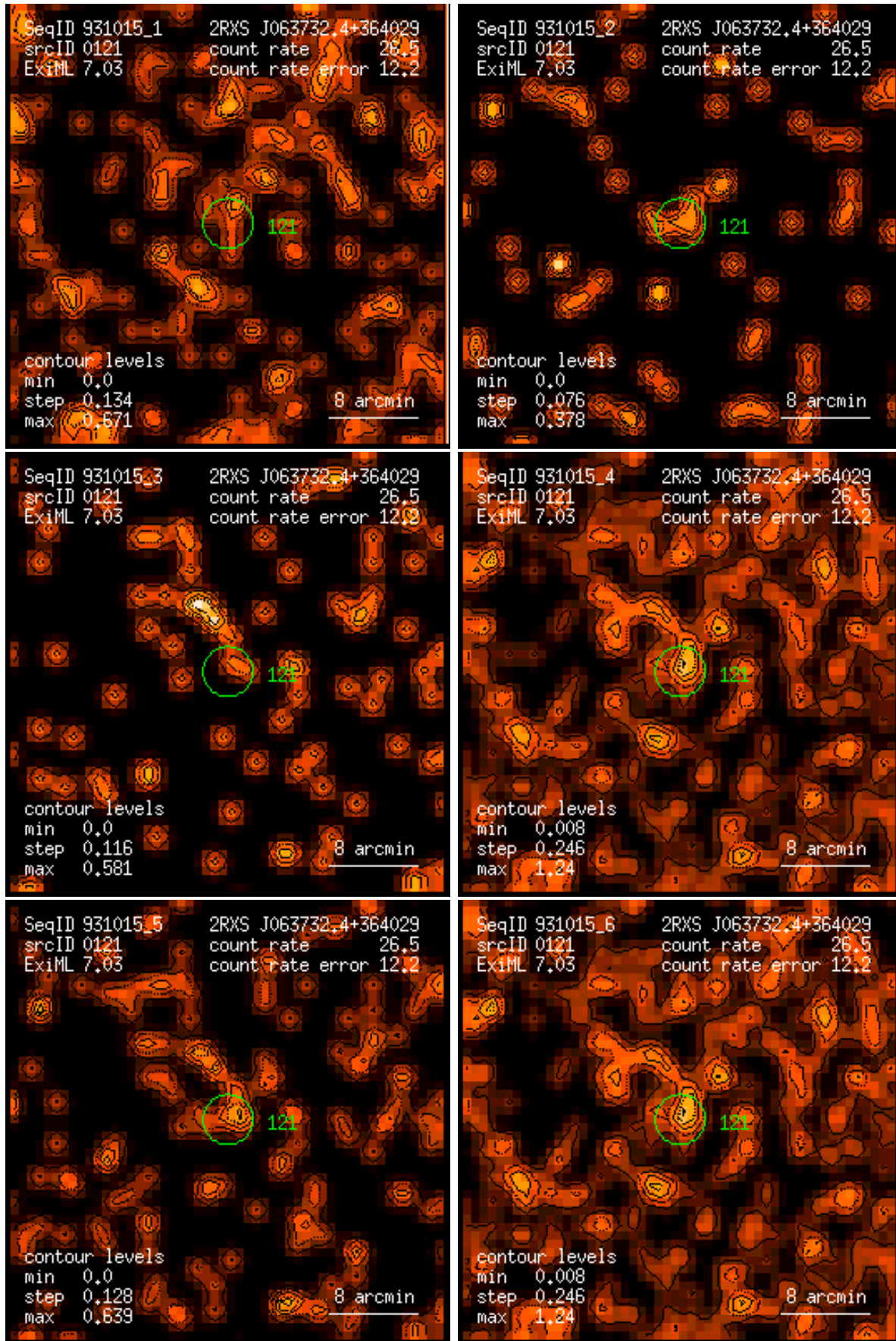
Figure 121: RASS 931015: detection 0121: band rate images, Gaussian filter: (1) PSPC channels 11 – 41, (2) 52 – 90, (3) 91 – 201, (4) 11 – 235, (5) 52 – 201, (6) 11 – 201. Broad band rates in counts/ks. Band rate contour levels in counts/ks/arcmin 2 .
