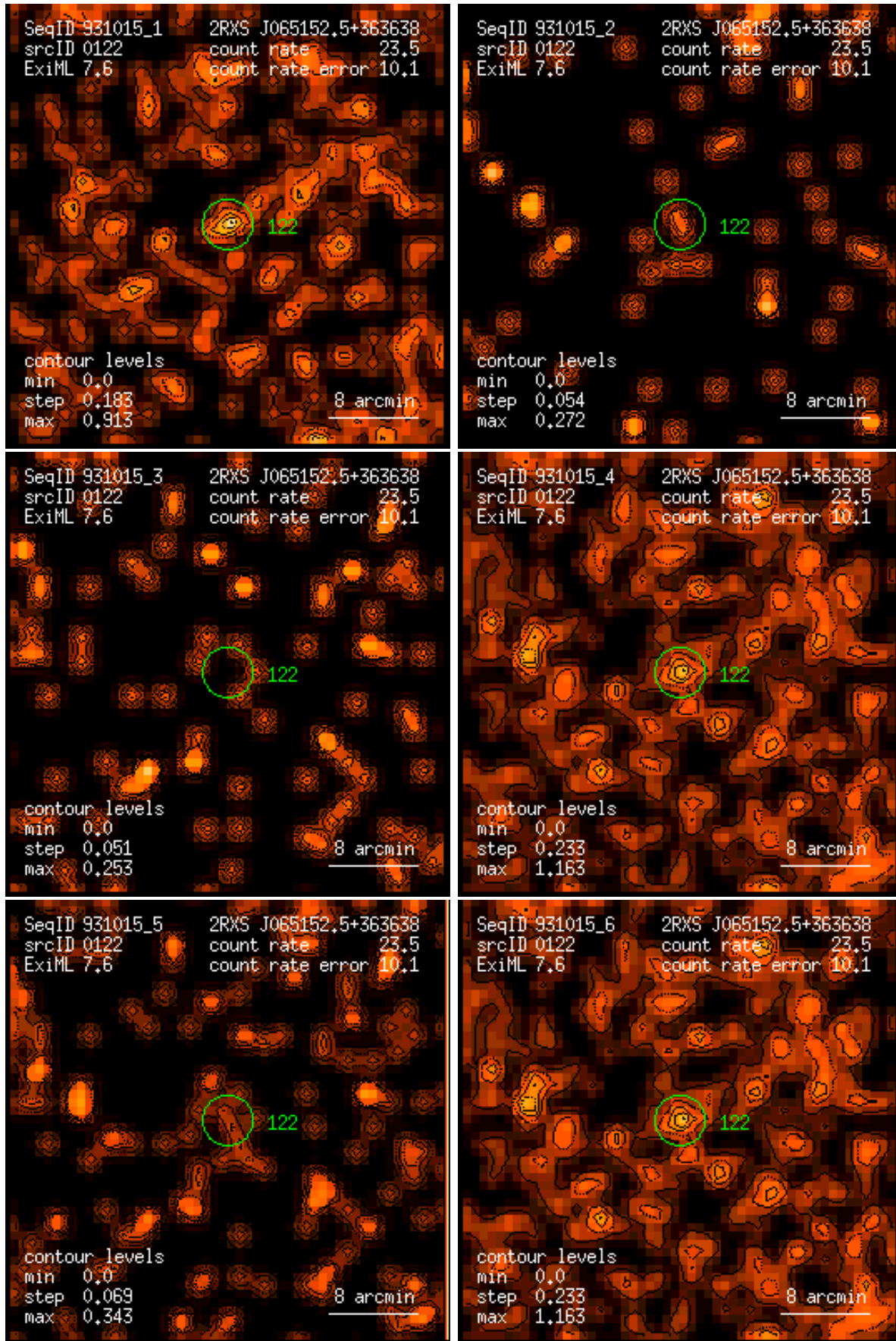
Figure 122: RASS 931015: detection 0122: band rate images, Gaussian filter: (1) PSPC channels 11 – 41, (2) 52 – 90, (3) 91 – 201, (4) 11 – 235, (5) 52 – 201, (6) 11 – 201. Broad band rates in counts/ks. Band rate contour levels in counts/ks/arcmin 2 .
