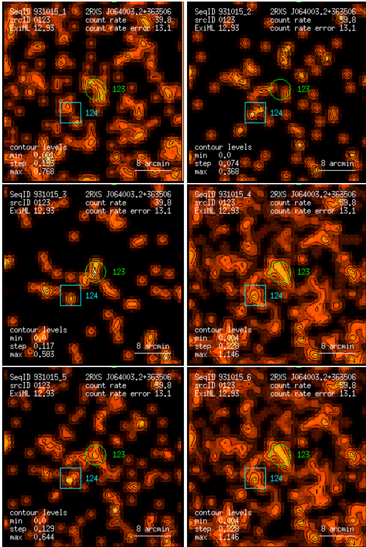
Figure 123: RASS 931015: detection 0123: band rate images, Gaussian filter: (1) PSPC channels 11 – 41, (2) 52 – 90, (3) 91 – 201, (4) 11 – 235, (5) 52 – 201, (6) 11 – 201. Broad band rates in counts/ks. Band rate contour levels in counts/ks/arcmin 2 .
