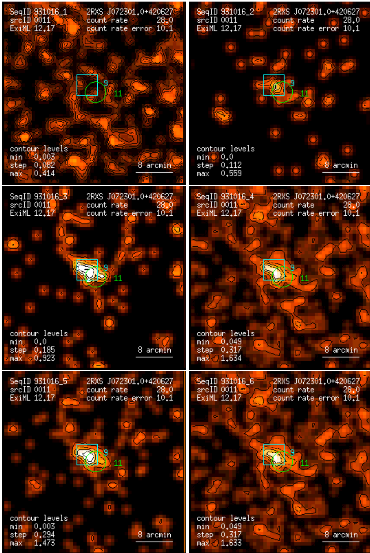
Figure 11: RASS 931016: detection 0011: band rate images, Gaussian filter: (1) PSPC channels 11 – 41, (2) 52 – 90, (3) 91 – 201, (4) 11 – 235, (5) 52 – 201, (6) 11 – 201. Broad band rates in counts/ks. Band rate contour levels in counts/ks/arcmin 2 .
