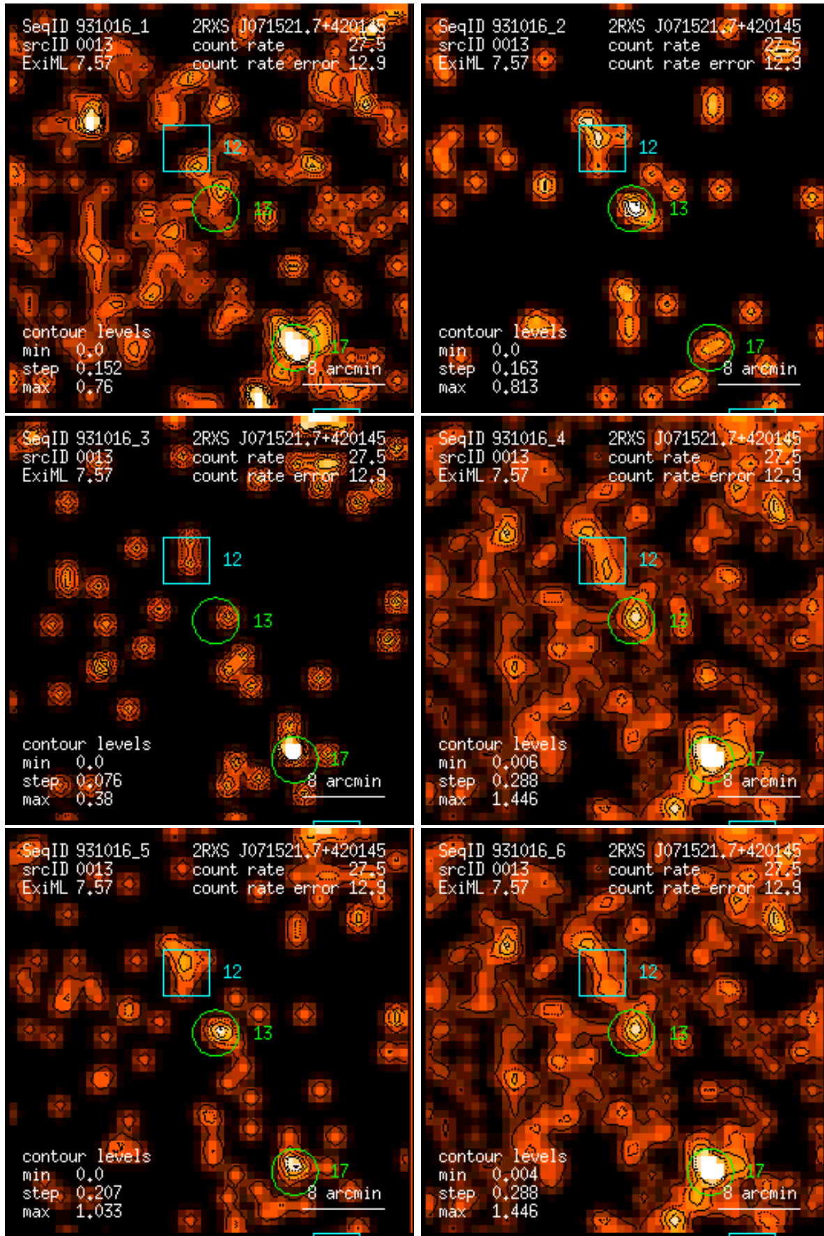
Figure 13: RASS 931016: detection 0013: band rate images, Gaussian filter: (1) PSPC channels 11 – 41, (2) 52 – 90, (3) 91 – 201, (4) 11 – 235, (5) 52 – 201, (6) 11 – 201. Broad band rates in counts/ks. Band rate contour levels in counts/ks/arcmin 2 .
