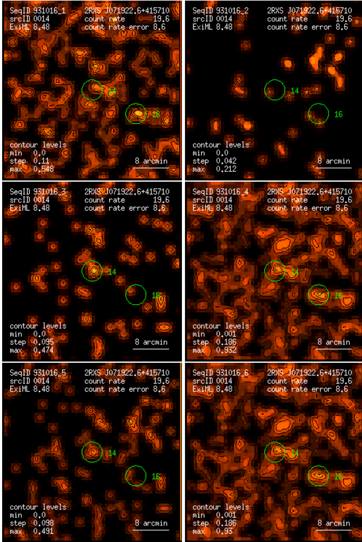
Figure 14: RASS 931016: detection 0014: band rate images, Gaussian filter: (1) PSPC channels 11 – 41, (2) 52 – 90, (3) 91 – 201, (4) 11 – 235, (5) 52 – 201, (6) 11 – 201. Broad band rates in counts/ks. Band rate contour levels in counts/ks/arcmin 2 .
