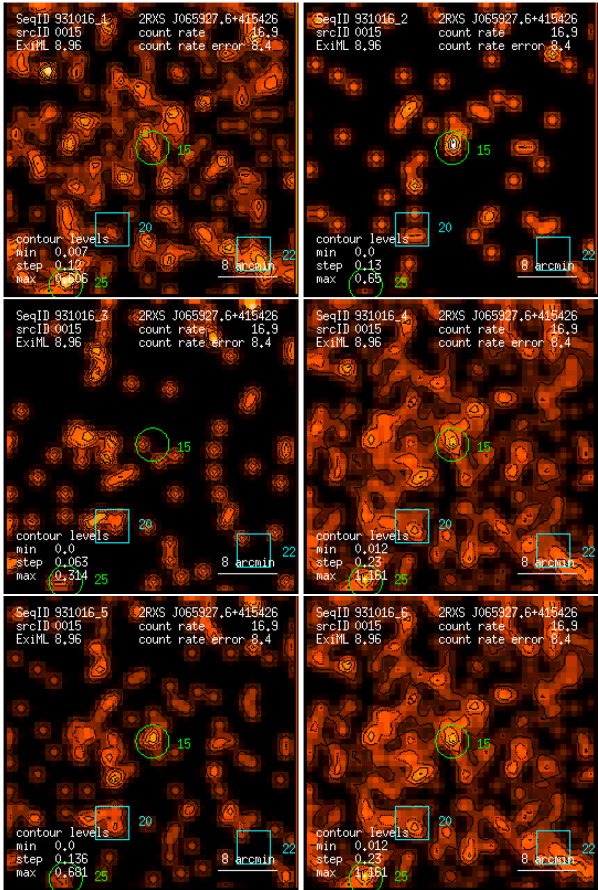
Figure 15: RASS 931016: detection 0015: band rate images, Gaussian filter: (1) PSPC channels 11 – 41, (2) 52 – 90, (3) 91 – 201, (4) 11 – 235, (5) 52 – 201, (6) 11 – 201. Broad band rates in counts/ks. Band rate contour levels in counts/ks/arcmin 2 .
