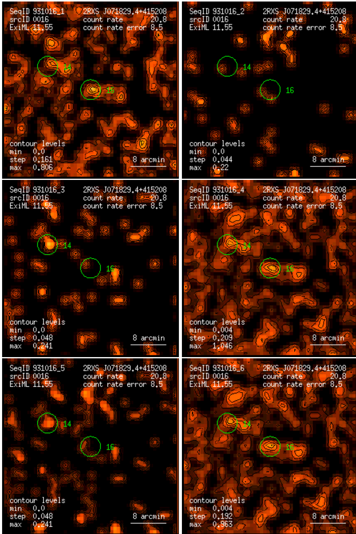
Figure 16: RASS 931016: detection 0016: band rate images, Gaussian filter: (1) PSPC channels 11 – 41, (2) 52 – 90, (3) 91 – 201, (4) 11 – 235, (5) 52 – 201, (6) 11 – 201. Broad band rates in counts/ks. Band rate contour levels in counts/ks/arcmin 2 .
