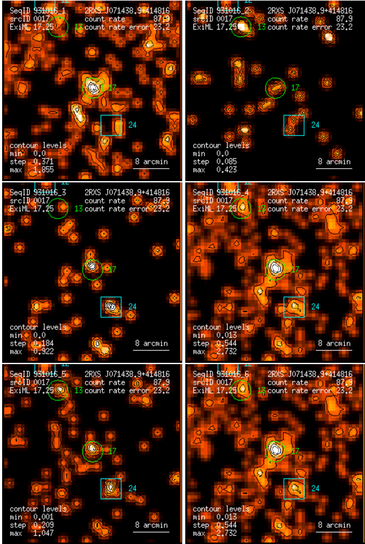
Figure 17: RASS 931016: detection 0017: band rate images, Gaussian filter: (1) PSPC channels 11 – 41, (2) 52 – 90, (3) 91 – 201, (4) 11 – 235, (5) 52 – 201, (6) 11 – 201. Broad band rates in counts/ks. Band rate contour levels in counts/ks/arcmin 2 .
