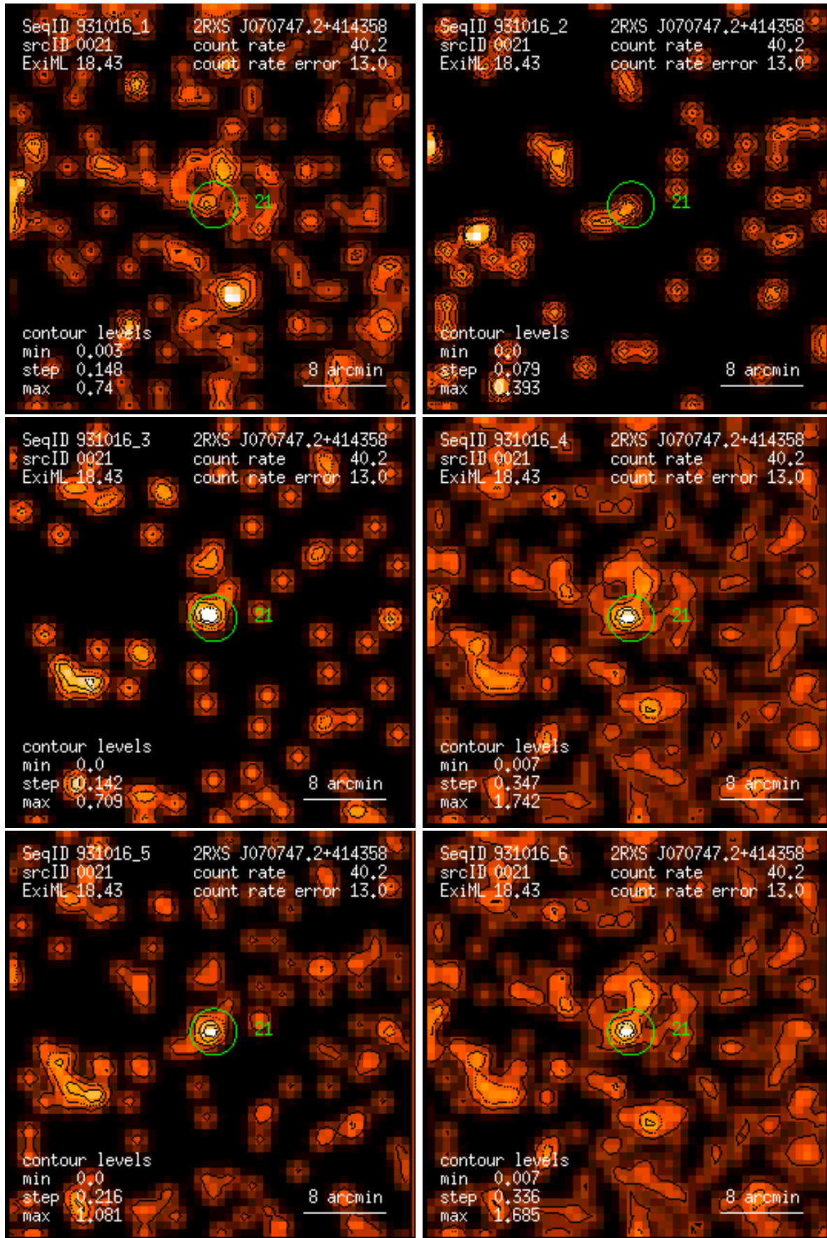
Figure 21: RASS 931016: detection 0021: band rate images, Gaussian filter: (1) PSPC channels 11 – 41, (2) 52 – 90, (3) 91 – 201, (4) 11 – 235, (5) 52 – 201, (6) 11 – 201. Broad band rates in counts/ks. Band rate contour levels in counts/ks/arcmin 2 .
