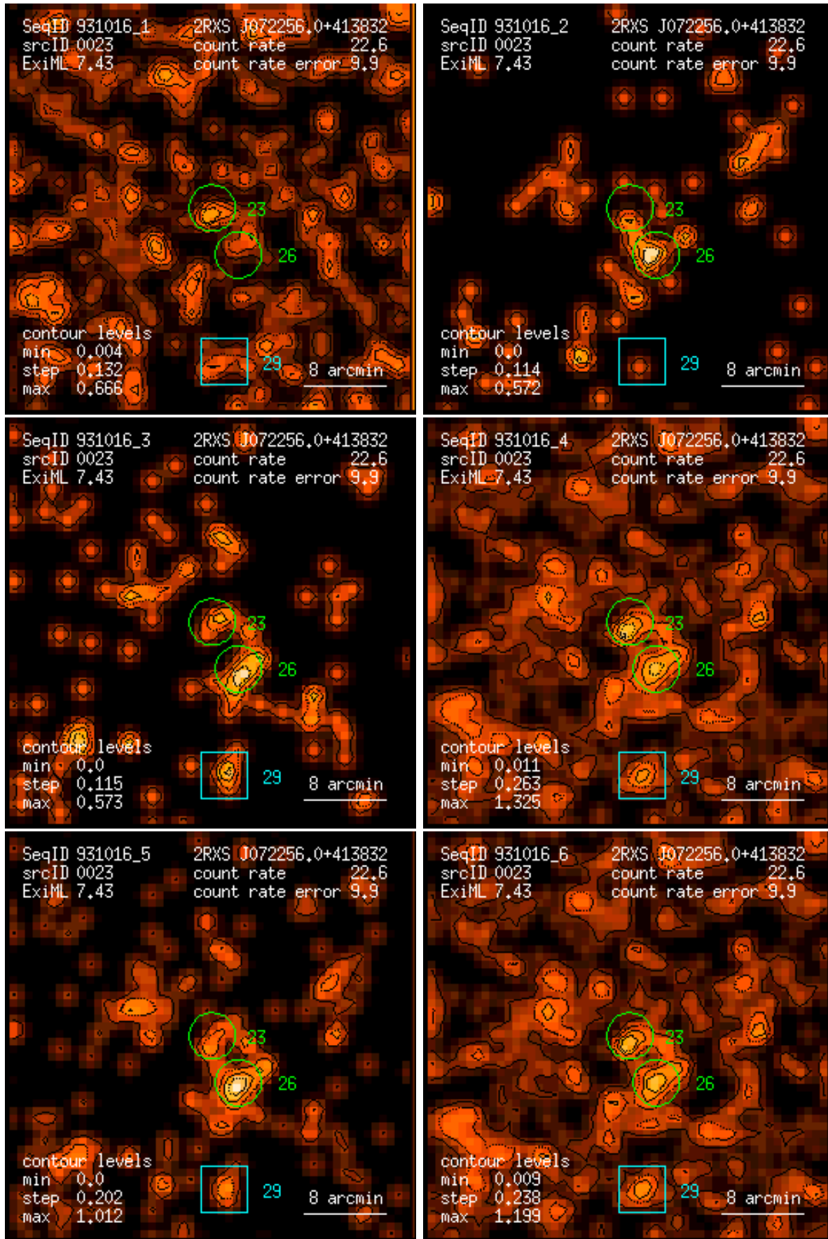
Figure 23: RASS 931016: detection 0023: band rate images, Gaussian filter: (1) PSPC channels 11 – 41, (2) 52 – 90, (3) 91 – 201, (4) 11 – 235, (5) 52 – 201, (6) 11 – 201. Broad band rates in counts/ks. Band rate contour levels in counts/ks/arcmin 2 .
