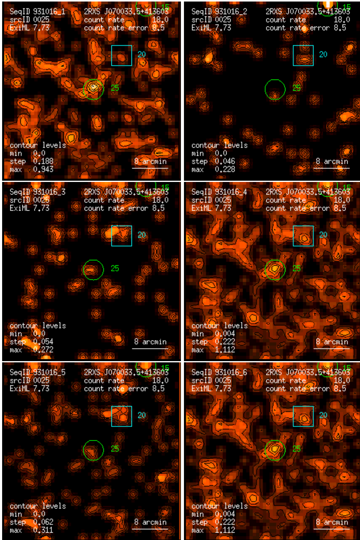
Figure 25: RASS 931016: detection 0025: band rate images, Gaussian filter: (1) PSPC channels 11 – 41, (2) 52 – 90, (3) 91 – 201, (4) 11 – 235, (5) 52 – 201, (6) 11 – 201. Broad band rates in counts/ks. Band rate contour levels in counts/ks/arcmin 2 .
