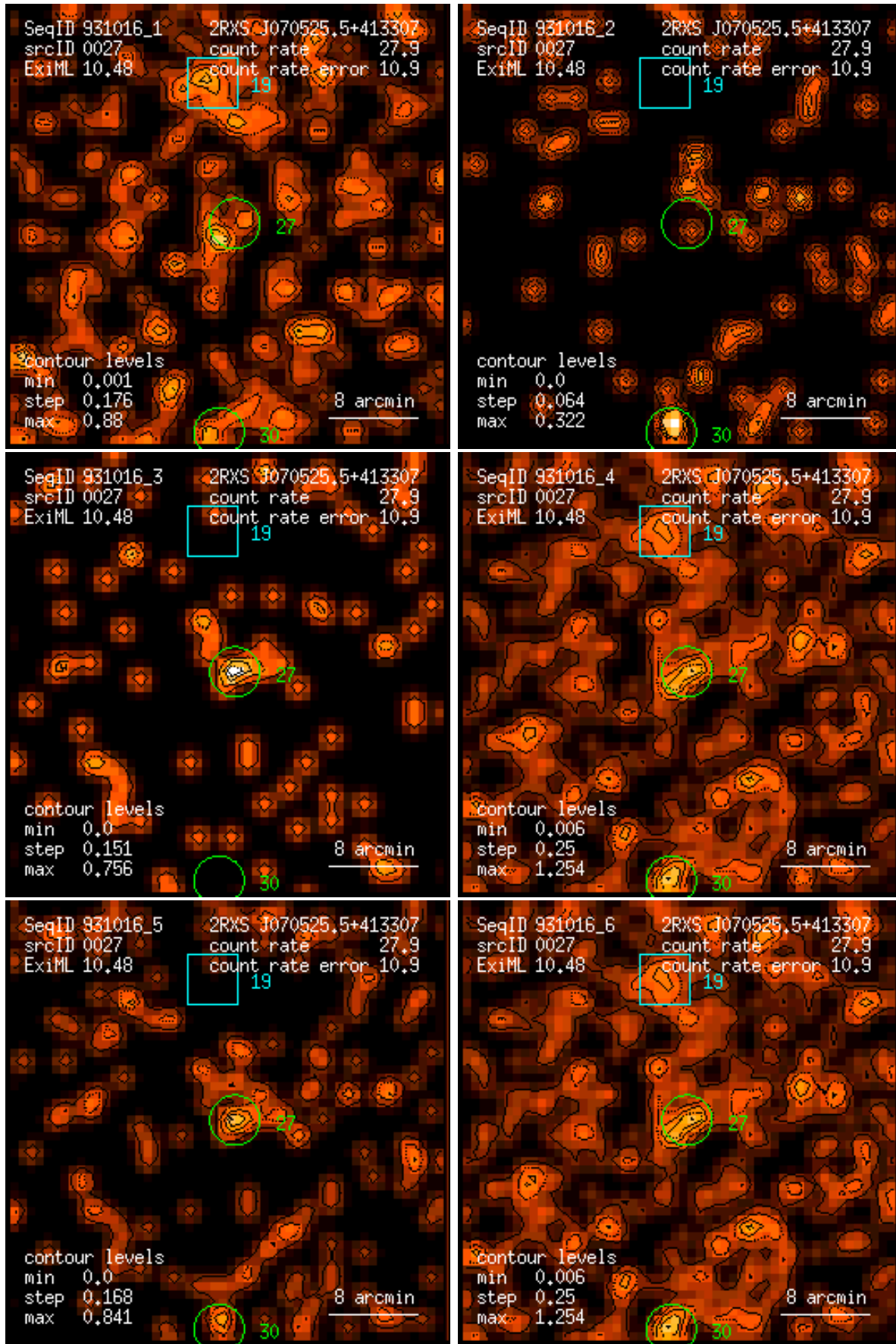
Figure 27: RASS 931016: detection 0027: band rate images, Gaussian filter: (1) PSPC channels 11 – 41, (2) 52 – 90, (3) 91 – 201, (4) 11 – 235, (5) 52 – 201, (6) 11 – 201. Broad band rates in counts/ks. Band rate contour levels in counts/ks/arcmin 2 .
