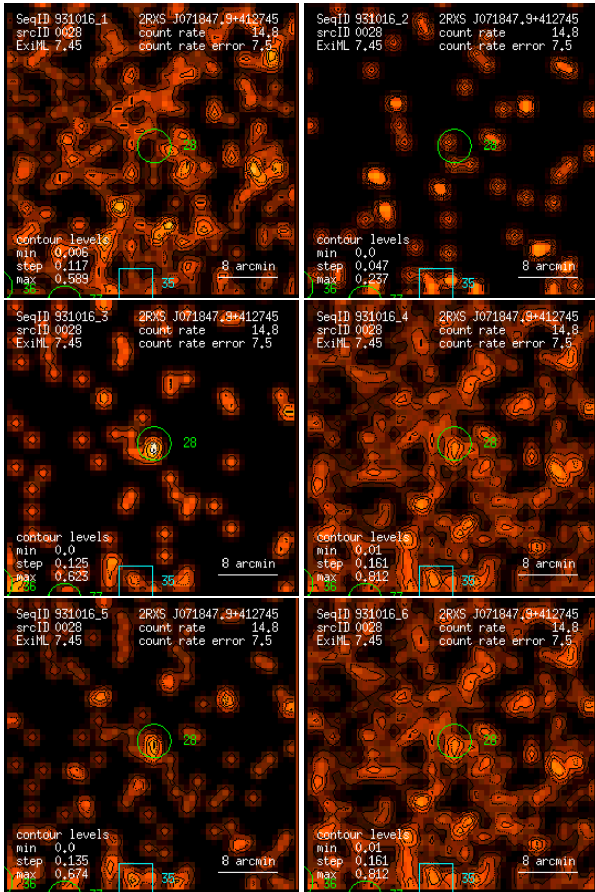
Figure 28: RASS 931016: detection 0028: band rate images, Gaussian filter: (1) PSPC channels 11 – 41, (2) 52 – 90, (3) 91 – 201, (4) 11 – 235, (5) 52 – 201, (6) 11 – 201. Broad band rates in counts/ks. Band rate contour levels in counts/ks/arcmin 2 .
