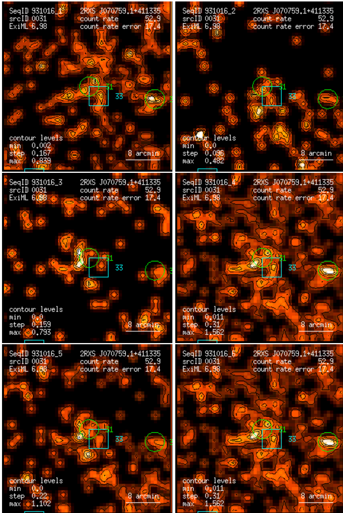
Figure 31: RASS 931016: detection 0031: band rate images, Gaussian filter: (1) PSPC channels 11 – 41, (2) 52 – 90, (3) 91 – 201, (4) 11 – 235, (5) 52 – 201, (6) 11 – 201. Broad band rates in counts/ks. Band rate contour levels in counts/ks/arcmin 2 .
