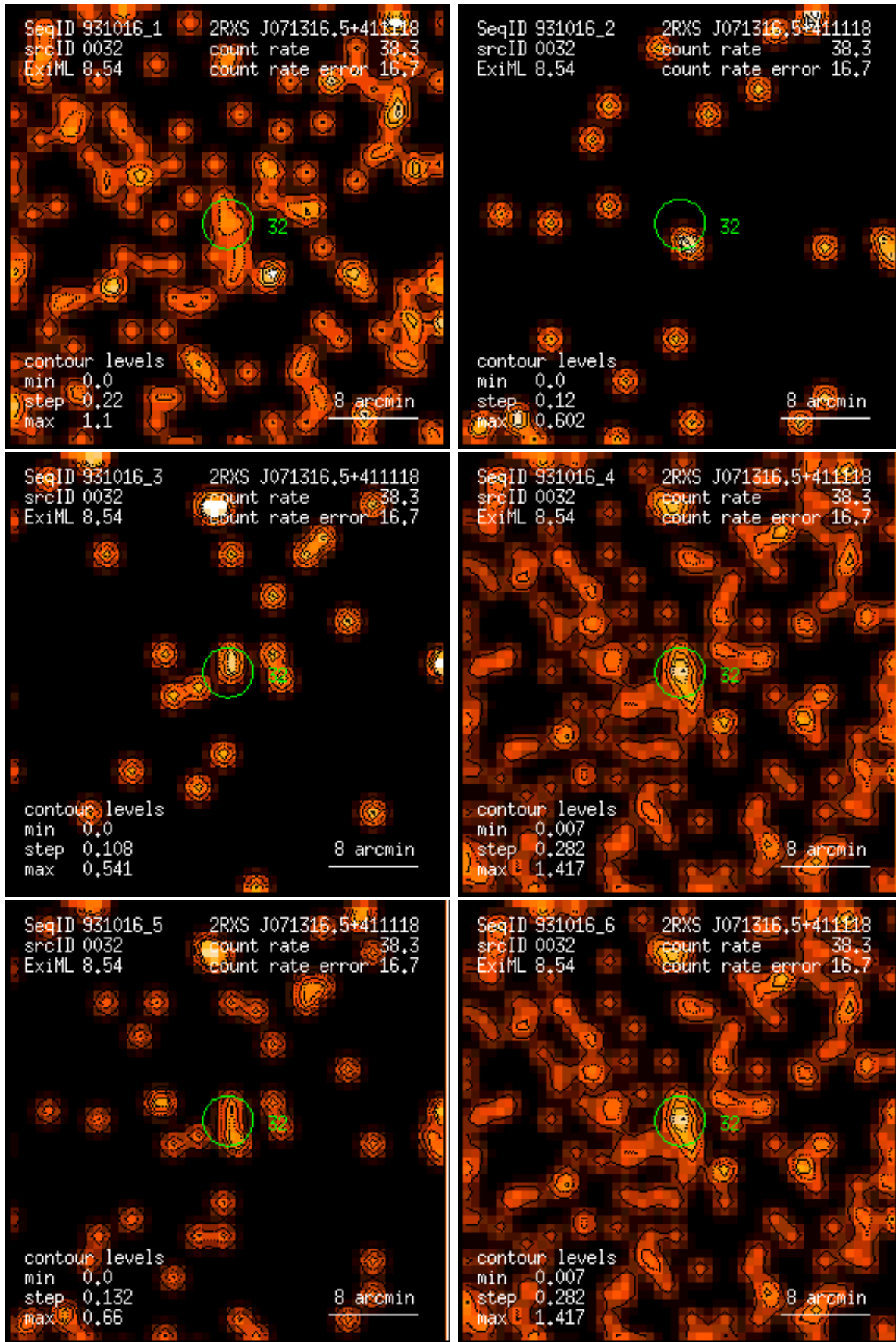
Figure 32: RASS 931016: detection 0032: band rate images, Gaussian filter: (1) PSPC channels 11 – 41, (2) 52 – 90, (3) 91 – 201, (4) 11 – 235, (5) 52 – 201, (6) 11 – 201. Broad band rates in counts/ks. Band rate contour levels in counts/ks/arcmin 2 .
