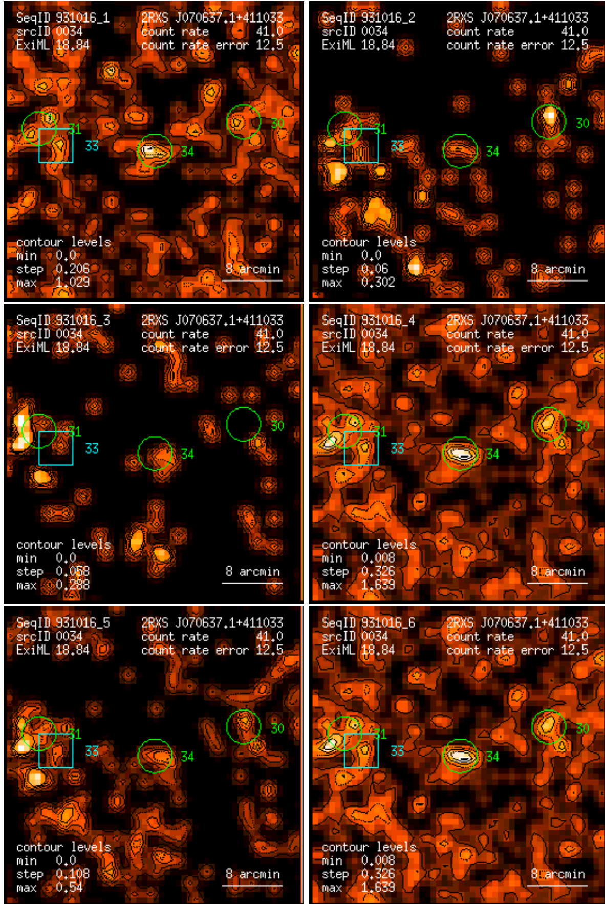
Figure 34: RASS 931016: detection 0034: band rate images, Gaussian filter: (1) PSPC channels 11 – 41, (2) 52 – 90, (3) 91 – 201, (4) 11 – 235, (5) 52 – 201, (6) 11 – 201. Broad band rates in counts/ks. Band rate contour levels in counts/ks/arcmin 2 .
