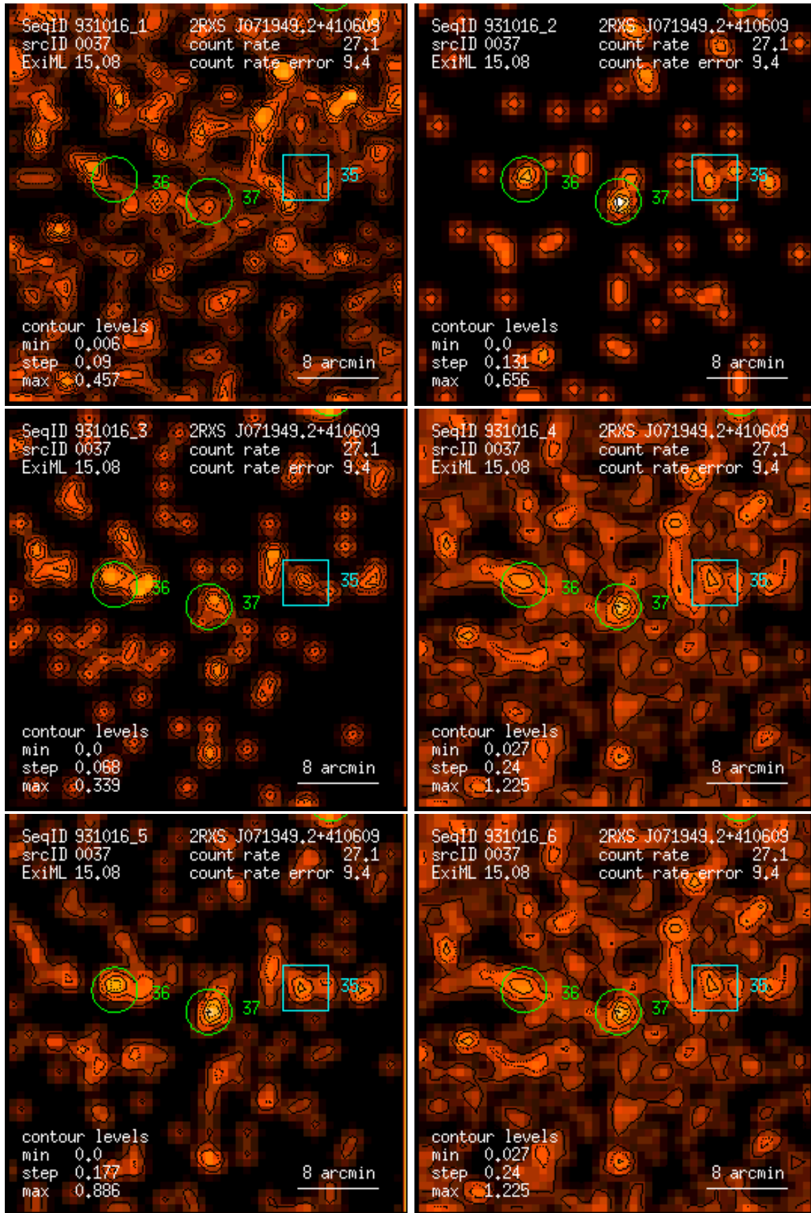
Figure 37: RASS 931016: detection 0037: band rate images, Gaussian filter: (1) PSPC channels 11 – 41, (2) 52 – 90, (3) 91 – 201, (4) 11 – 235, (5) 52 – 201, (6) 11 – 201. Broad band rates in counts/ks. Band rate contour levels in counts/ks/arcmin 2 .
