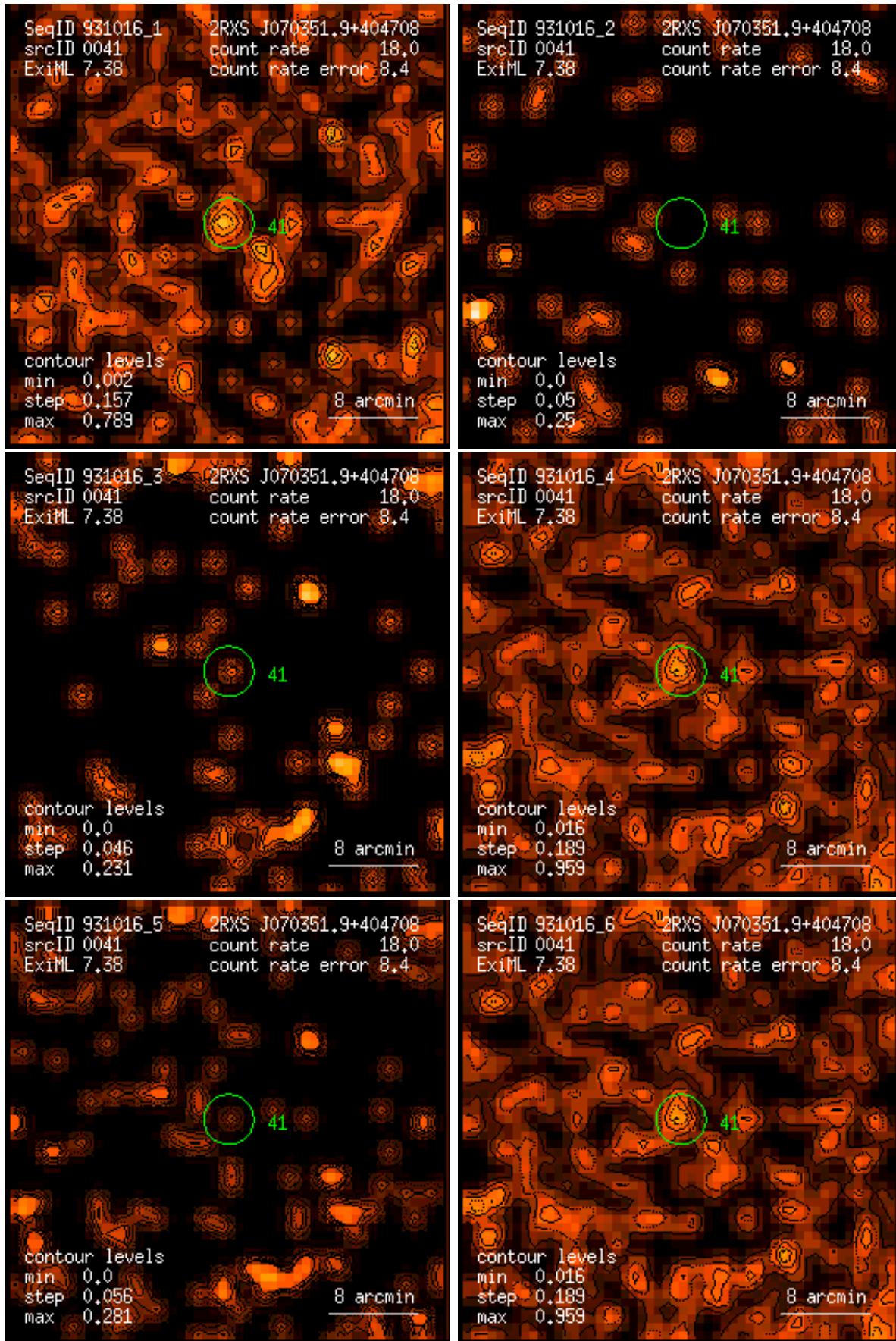
Figure 41: RASS 931016: detection 0041: band rate images, Gaussian filter: (1) PSPC channels 11 – 41, (2) 52 – 90, (3) 91 – 201, (4) 11 – 235, (5) 52 – 201, (6) 11 – 201. Broad band rates in counts/ks. Band rate contour levels in counts/ks/arcmin 2 .
