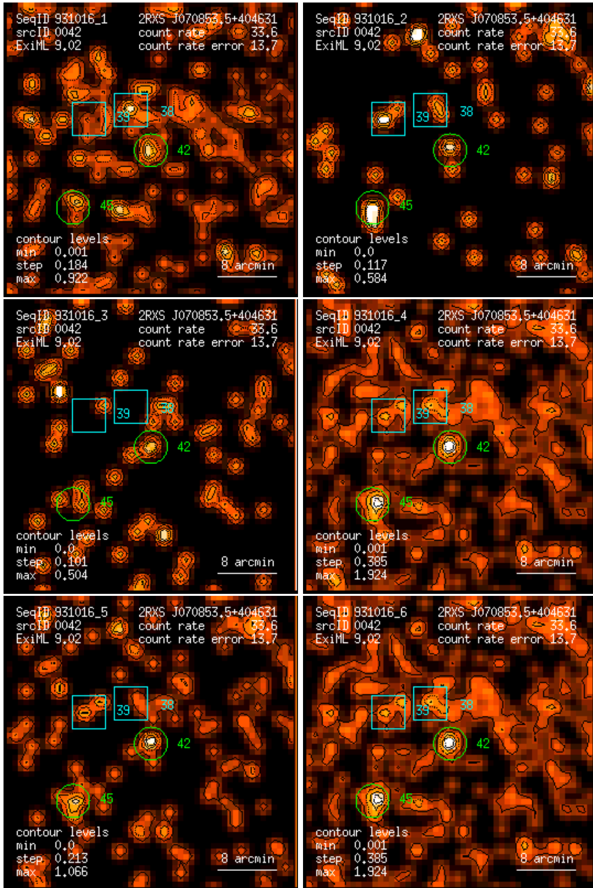
Figure 42: RASS 931016: detection 0042: band rate images, Gaussian filter: (1) PSPC channels 11 – 41, (2) 52 – 90, (3) 91 – 201, (4) 11 – 235, (5) 52 – 201, (6) 11 – 201. Broad band rates in counts/ks. Band rate contour levels in counts/ks/arcmin 2 .
