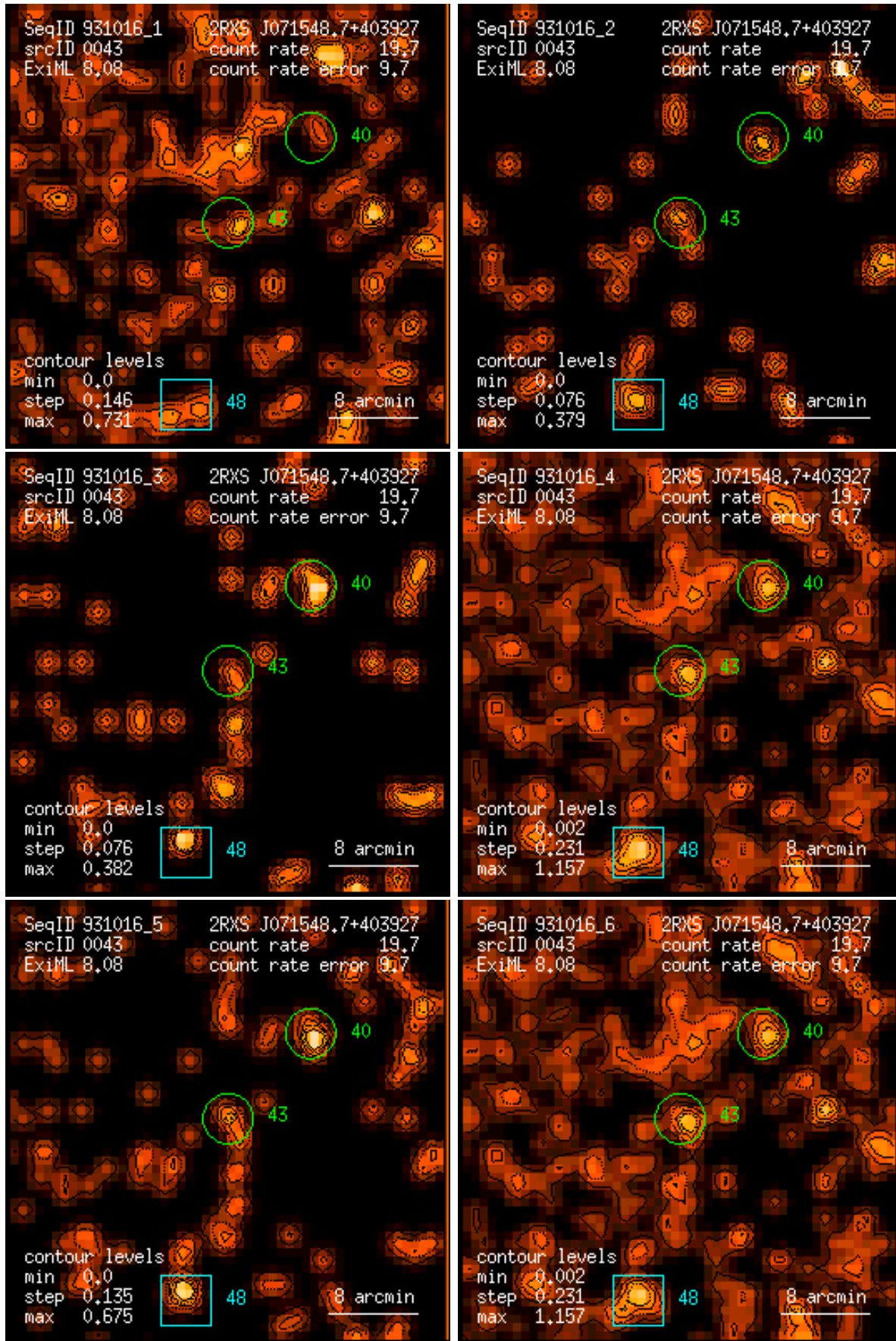
Figure 43: RASS 931016: detection 0043: band rate images, Gaussian filter: (1) PSPC channels 11 – 41, (2) 52 – 90, (3) 91 – 201, (4) 11 – 235, (5) 52 – 201, (6) 11 – 201. Broad band rates in counts/ks. Band rate contour levels in counts/ks/arcmin 2 .
