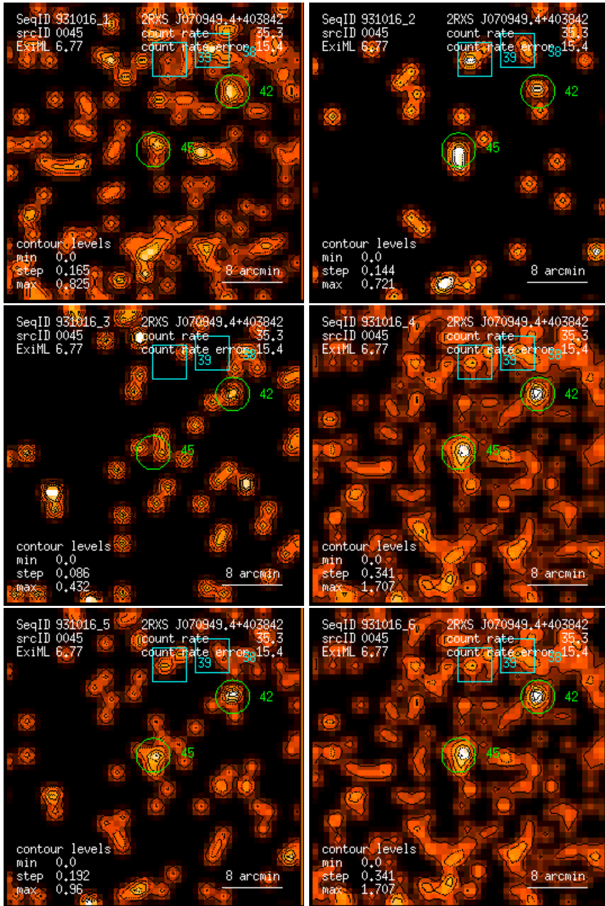
Figure 45: RASS 931016: detection 0045: band rate images, Gaussian filter: (1) PSPC channels 11 – 41, (2) 52 – 90, (3) 91 – 201, (4) 11 – 235, (5) 52 – 201, (6) 11 – 201. Broad band rates in counts/ks. Band rate contour levels in counts/ks/arcmin 2 .
