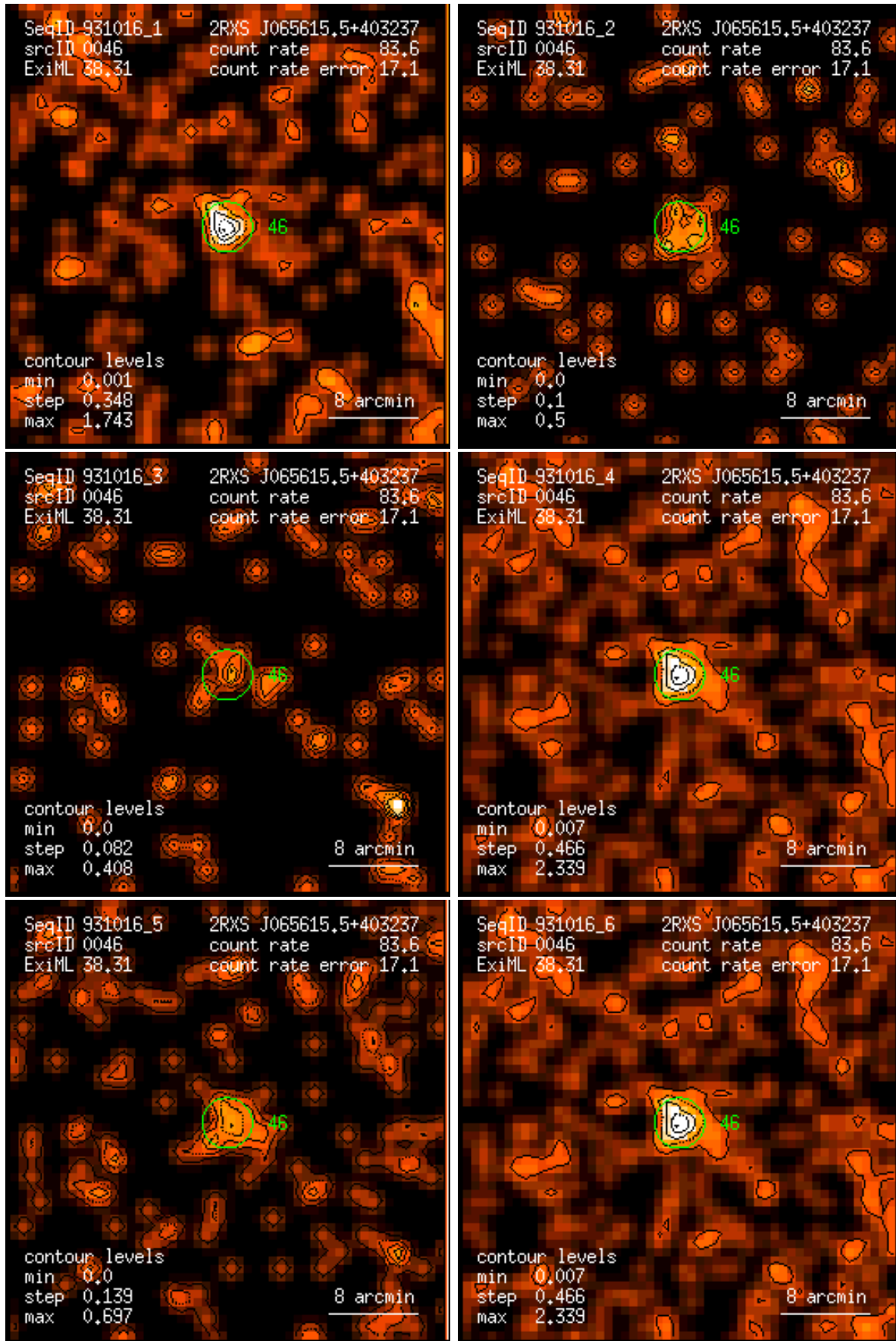
Figure 46: RASS 931016: detection 0046: band rate images, Gaussian filter: (1) PSPC channels 11 – 41, (2) 52 – 90, (3) 91 – 201, (4) 11 – 235, (5) 52 – 201, (6) 11 – 201. Broad band rates in counts/ks. Band rate contour levels in counts/ks/arcmin 2 .
