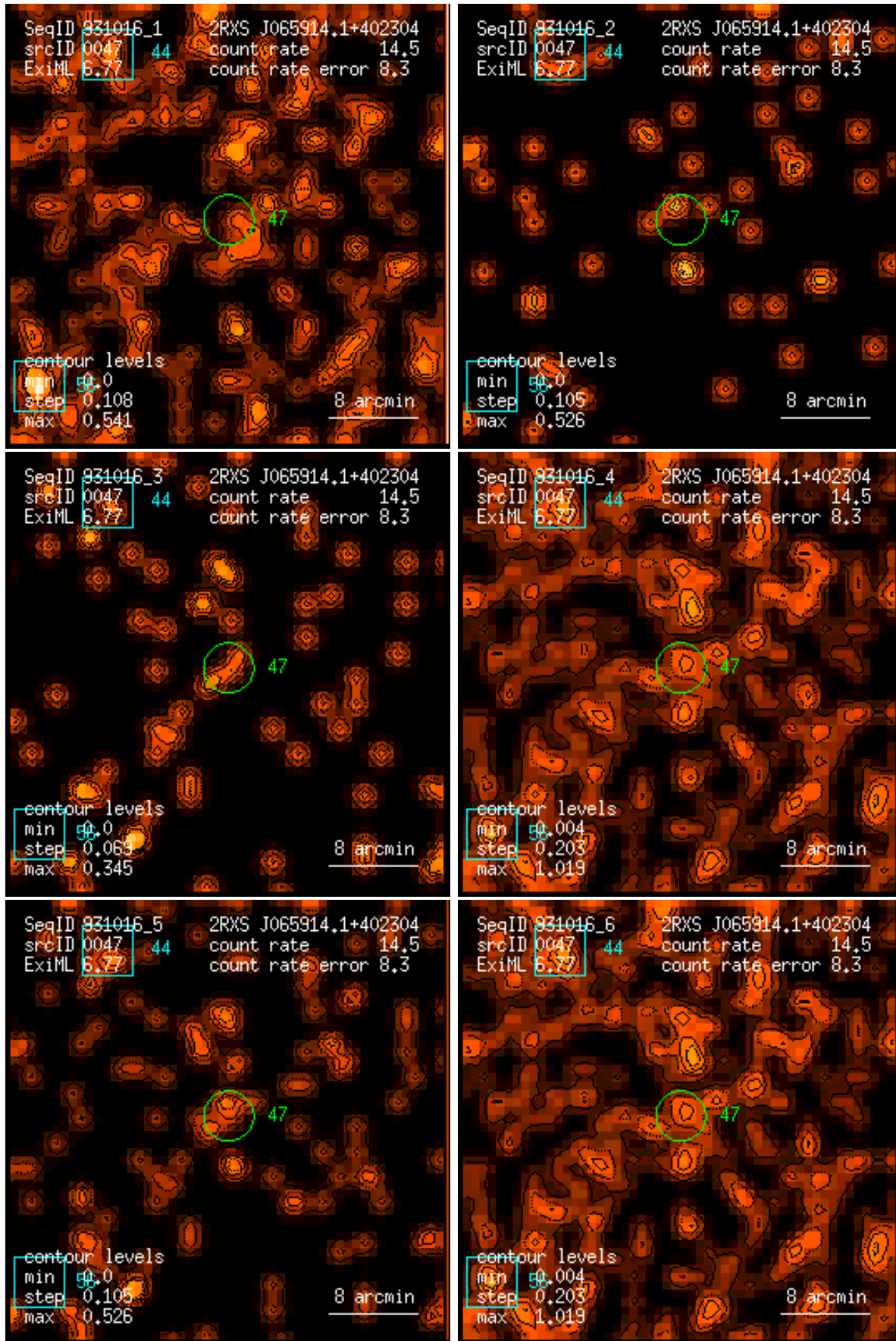
Figure 47: RASS 931016: detection 0047: band rate images, Gaussian filter: (1) PSPC channels 11 – 41, (2) 52 – 90, (3) 91 – 201, (4) 11 – 235, (5) 52 – 201, (6) 11 – 201. Broad band rates in counts/ks. Band rate contour levels in counts/ks/arcmin 2 .
