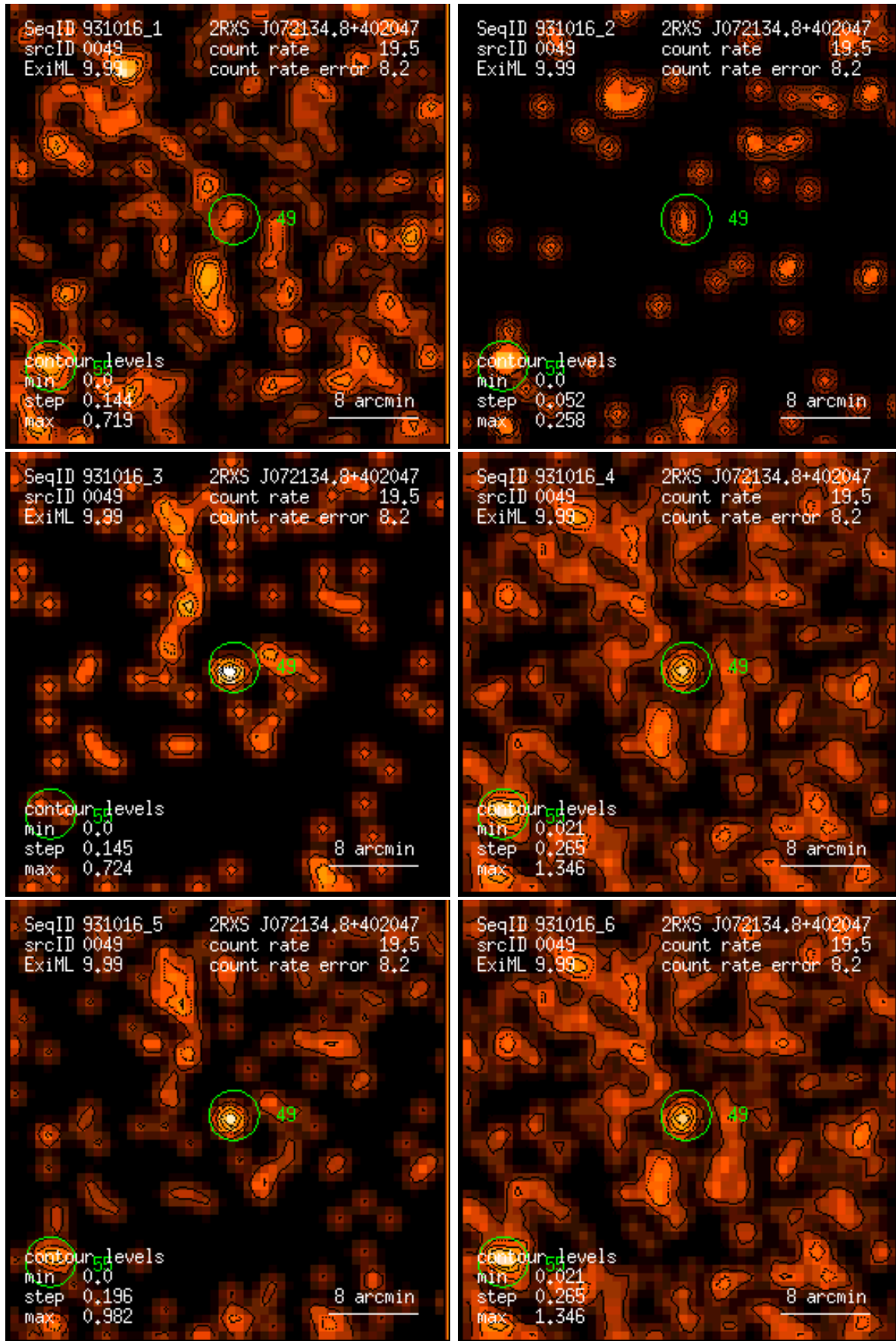
Figure 49: RASS 931016: detection 0049: band rate images, Gaussian filter: (1) PSPC channels 11 – 41, (2) 52 – 90, (3) 91 – 201, (4) 11 – 235, (5) 52 – 201, (6) 11 – 201. Broad band rates in counts/ks. Band rate contour levels in counts/ks/arcmin 2 .
