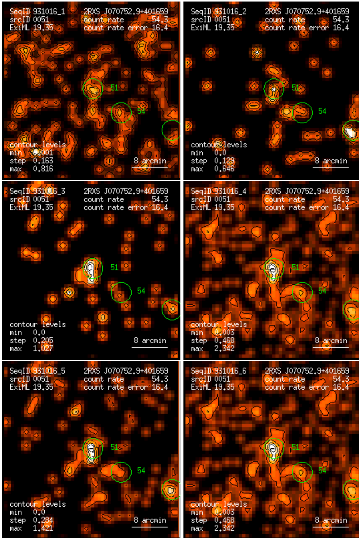
Figure 51: RASS 931016: detection 0051: band rate images, Gaussian filter: (1) PSPC channels 11 – 41, (2) 52 – 90, (3) 91 – 201, (4) 11 – 235, (5) 52 – 201, (6) 11 – 201. Broad band rates in counts/ks. Band rate contour levels in counts/ks/arcmin 2 .
