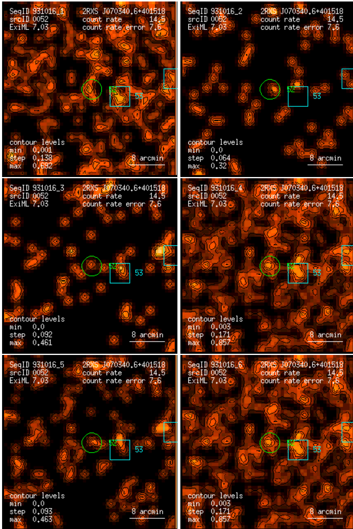
Figure 52: RASS 931016: detection 0052: band rate images, Gaussian filter: (1) PSPC channels 11 – 41, (2) 52 – 90, (3) 91 – 201, (4) 11 – 235, (5) 52 – 201, (6) 11 – 201. Broad band rates in counts/ks. Band rate contour levels in counts/ks/arcmin 2 .
