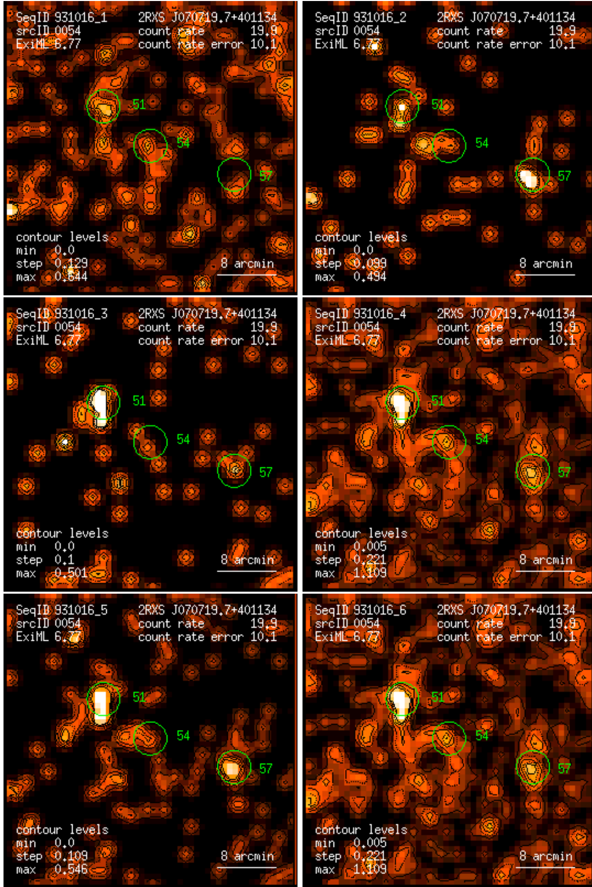
Figure 54: RASS 931016: detection 0054: band rate images, Gaussian filter: (1) PSPC channels 11 – 41, (2) 52 – 90, (3) 91 – 201, (4) 11 – 235, (5) 52 – 201, (6) 11 – 201. Broad band rates in counts/ks. Band rate contour levels in counts/ks/arcmin 2 .
