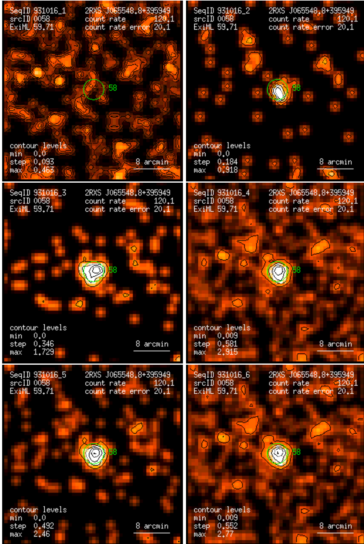
Figure 58: RASS 931016: detection 0058: band rate images, Gaussian filter: (1) PSPC channels 11 – 41, (2) 52 – 90, (3) 91 – 201, (4) 11 – 235, (5) 52 – 201, (6) 11 – 201. Broad band rates in counts/ks. Band rate contour levels in counts/ks/arcmin 2 .
