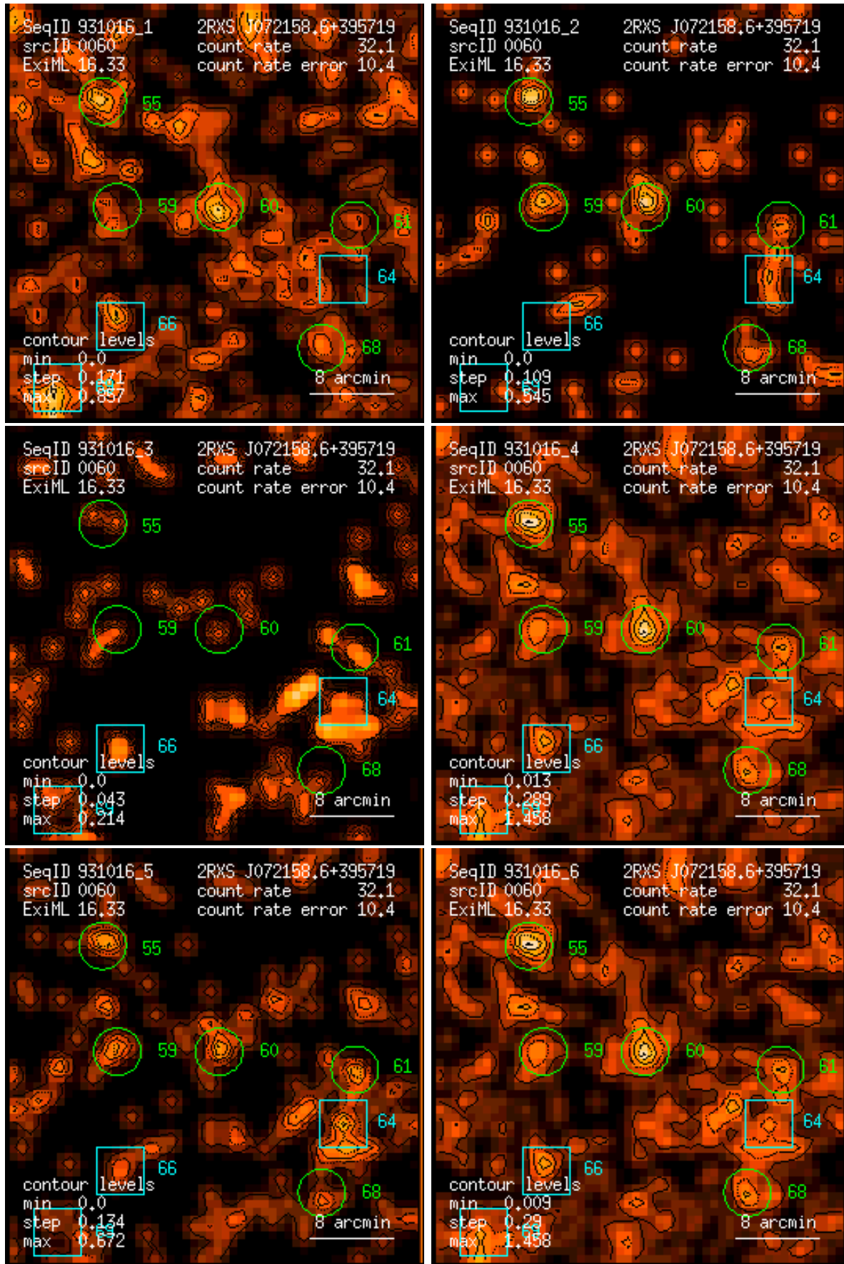
Figure 60: RASS 931016: detection 0060: band rate images, Gaussian filter: (1) PSPC channels 11 – 41, (2) 52 – 90, (3) 91 – 201, (4) 11 – 235, (5) 52 – 201, (6) 11 – 201. Broad band rates in counts/ks. Band rate contour levels in counts/ks/arcmin 2 .
