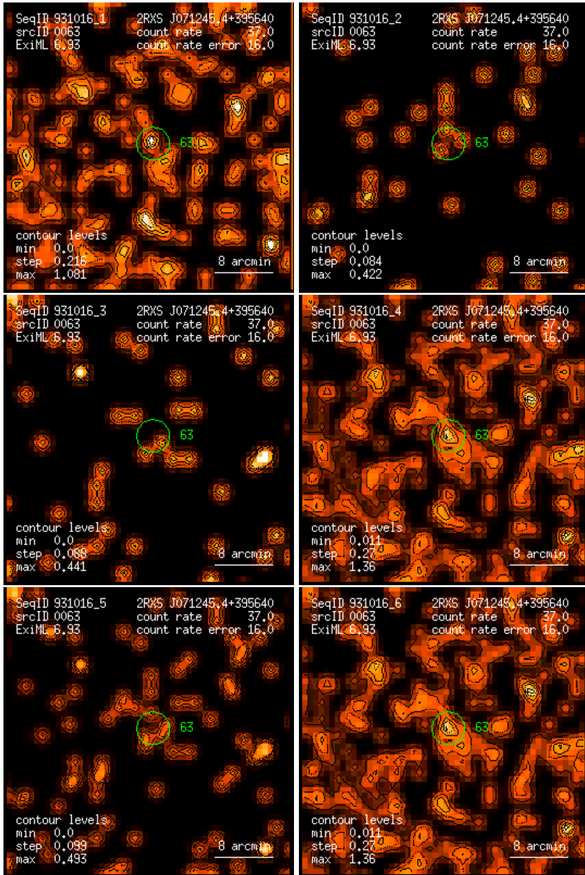
Figure 63: RASS 931016: detection 0063: band rate images, Gaussian filter: (1) PSPC channels 11 – 41, (2) 52 – 90, (3) 91 – 201, (4) 11 – 235, (5) 52 – 201, (6) 11 – 201. Broad band rates in counts/ks. Band rate contour levels in counts/ks/arcmin 2 .
