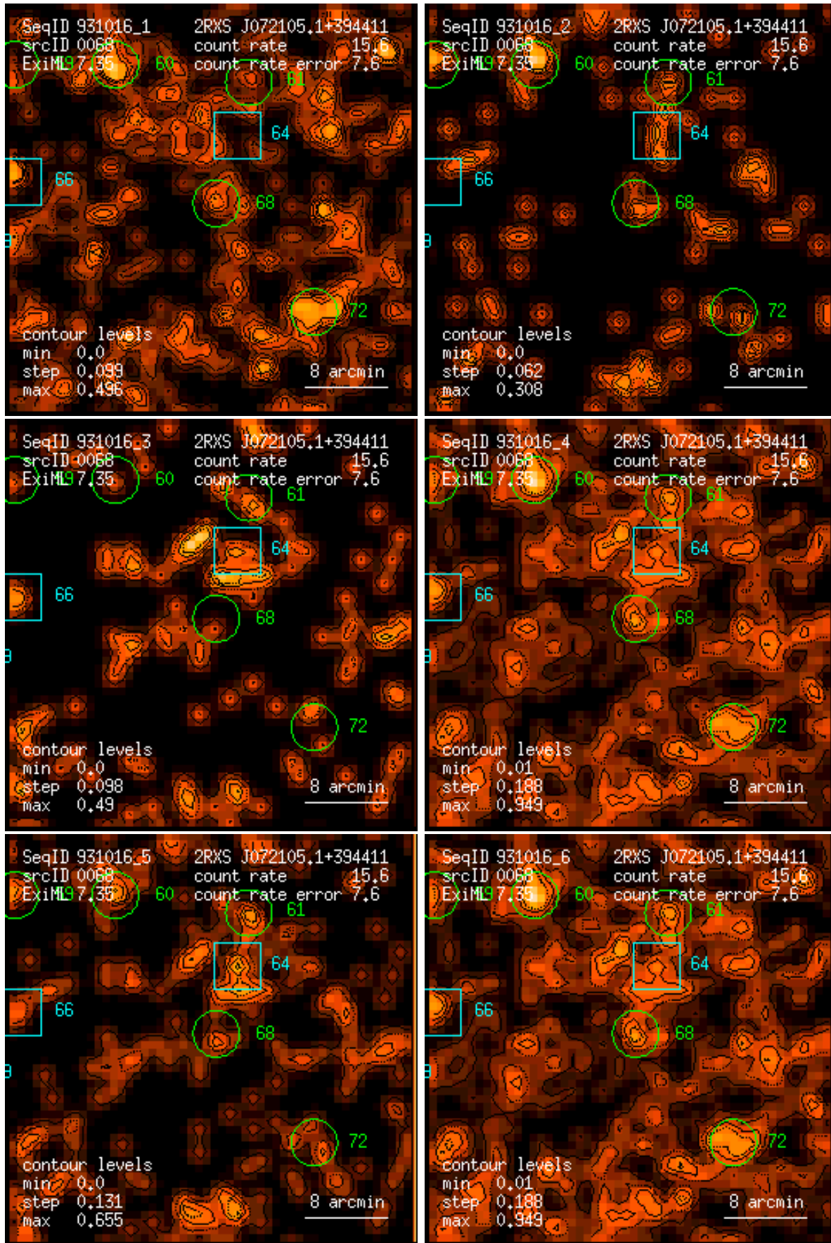
Figure 68: RASS 931016: detection 0068: band rate images, Gaussian filter: (1) PSPC channels 11 – 41, (2) 52 – 90, (3) 91 – 201, (4) 11 – 235, (5) 52 – 201, (6) 11 – 201. Broad band rates in counts/ks. Band rate contour levels in counts/ks/arcmin 2 .
