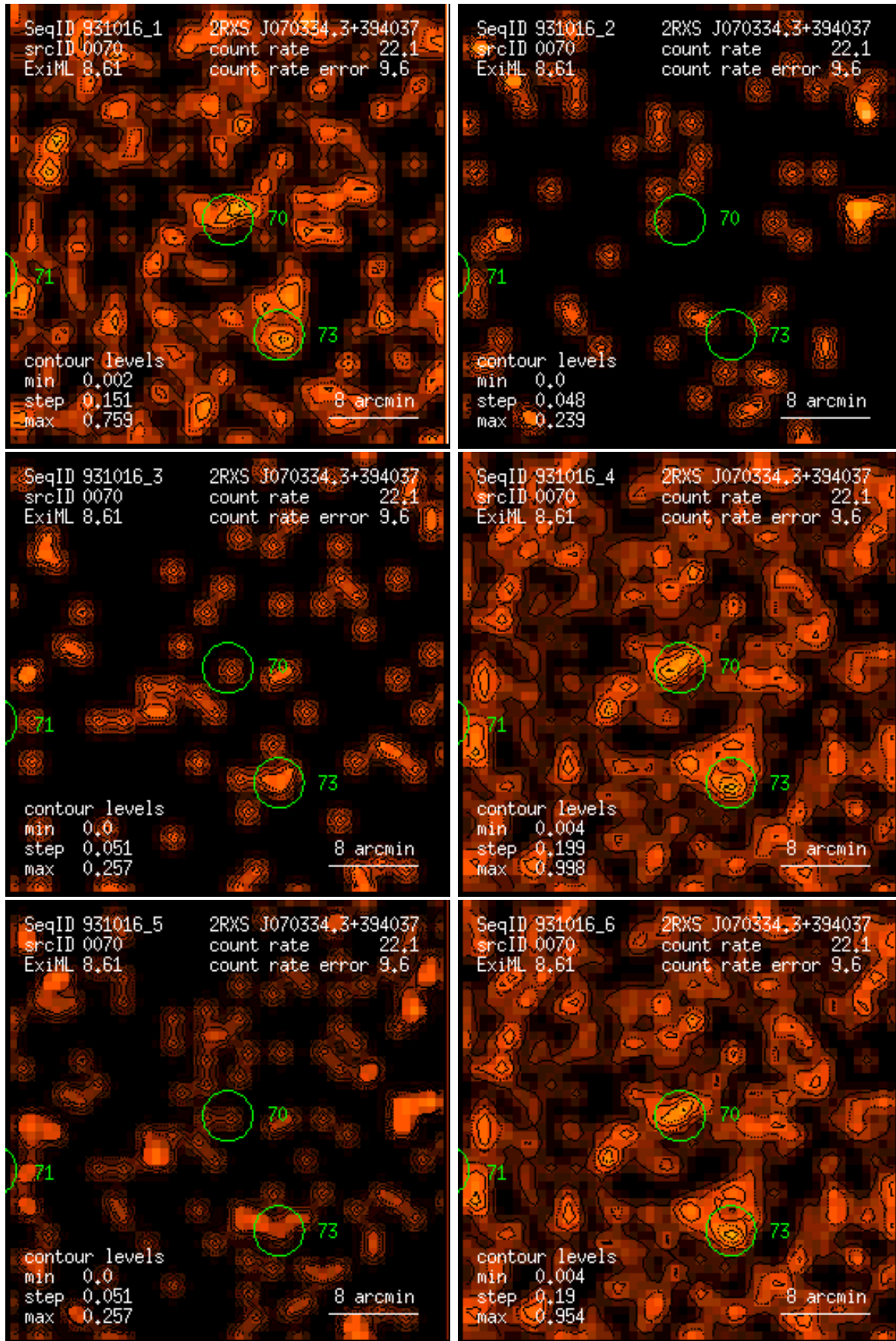
Figure 70: RASS 931016: detection 0070: band rate images, Gaussian filter: (1) PSPC channels 11 – 41, (2) 52 – 90, (3) 91 – 201, (4) 11 – 235, (5) 52 – 201, (6) 11 – 201. Broad band rates in counts/ks. Band rate contour levels in counts/ks/arcmin 2 .
