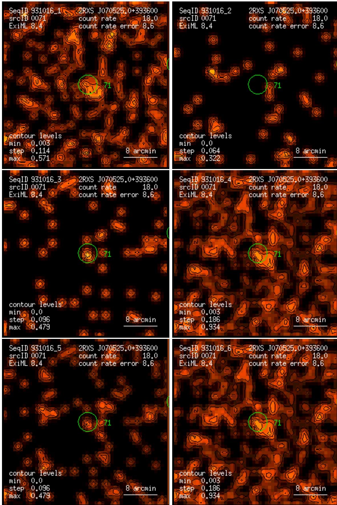
Figure 71: RASS 931016: detection 0071: band rate images, Gaussian filter: (1) PSPC channels 11 – 41, (2) 52 – 90, (3) 91 – 201, (4) 11 – 235, (5) 52 – 201, (6) 11 – 201. Broad band rates in counts/ks. Band rate contour levels in counts/ks/arcmin 2 .
