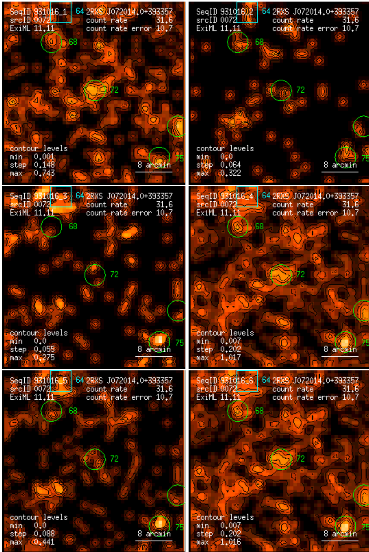
Figure 72: RASS 931016: detection 0072: band rate images, Gaussian filter: (1) PSPC channels 11 – 41, (2) 52 – 90, (3) 91 – 201, (4) 11 – 235, (5) 52 – 201, (6) 11 – 201. Broad band rates in counts/ks. Band rate contour levels in counts/ks/arcmin 2 .
