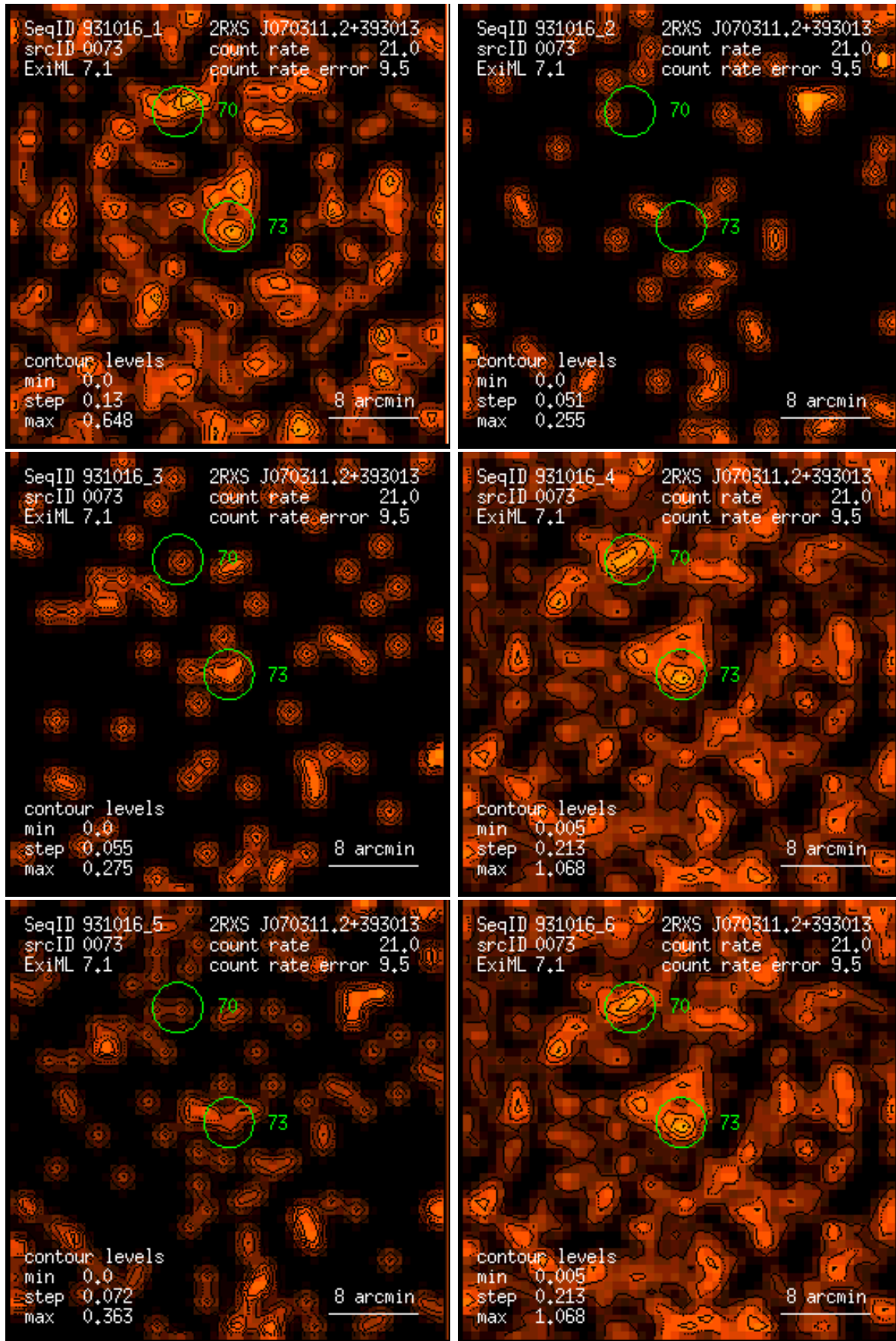
Figure 73: RASS 931016: detection 0073: band rate images, Gaussian filter: (1) PSPC channels 11 – 41, (2) 52 – 90, (3) 91 – 201, (4) 11 – 235, (5) 52 – 201, (6) 11 – 201. Broad band rates in counts/ks. Band rate contour levels in counts/ks/arcmin 2 .
