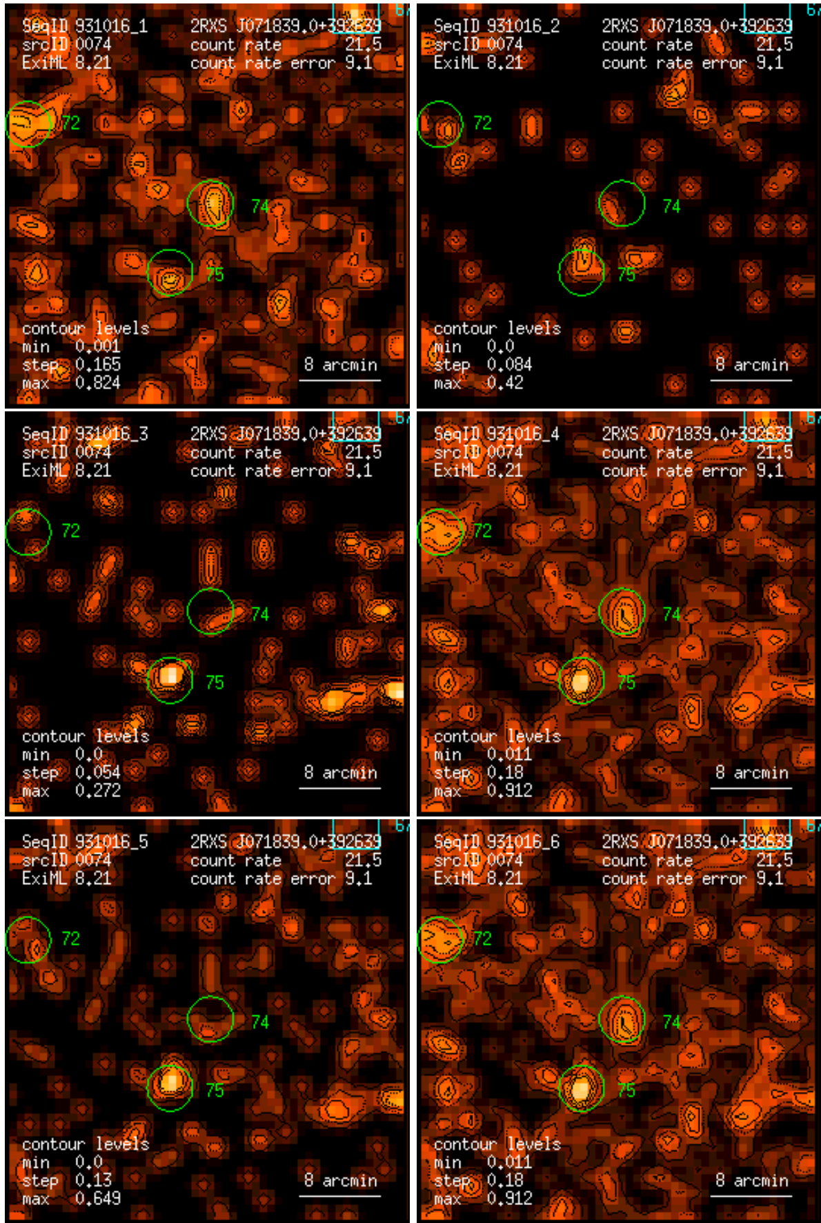
Figure 74: RASS 931016: detection 0074: band rate images, Gaussian filter: (1) PSPC channels 11 – 41, (2) 52 – 90, (3) 91 – 201, (4) 11 – 235, (5) 52 – 201, (6) 11 – 201. Broad band rates in counts/ks. Band rate contour levels in counts/ks/arcmin 2 .
