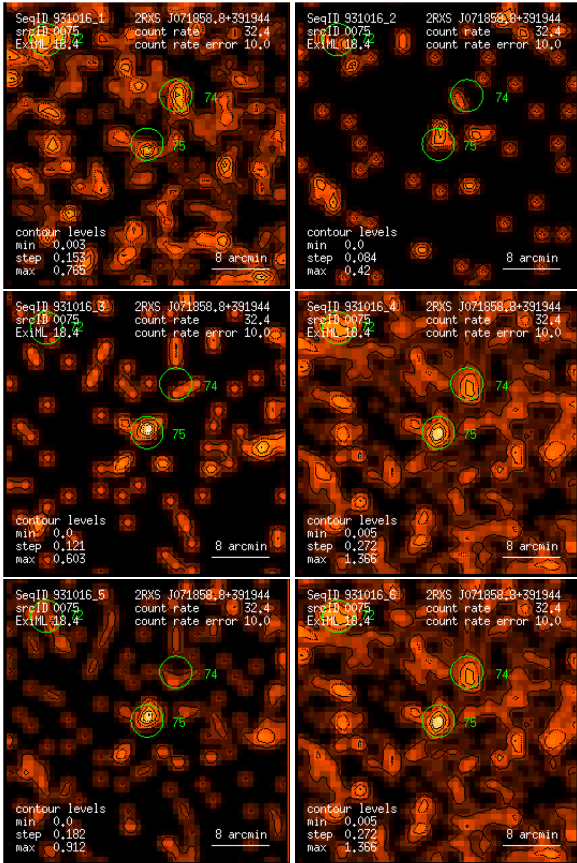
Figure 75: RASS 931016: detection 0075: band rate images, Gaussian filter: (1) PSPC channels 11 – 41, (2) 52 – 90, (3) 91 – 201, (4) 11 – 235, (5) 52 – 201, (6) 11 – 201. Broad band rates in counts/ks. Band rate contour levels in counts/ks/arcmin 2 .
