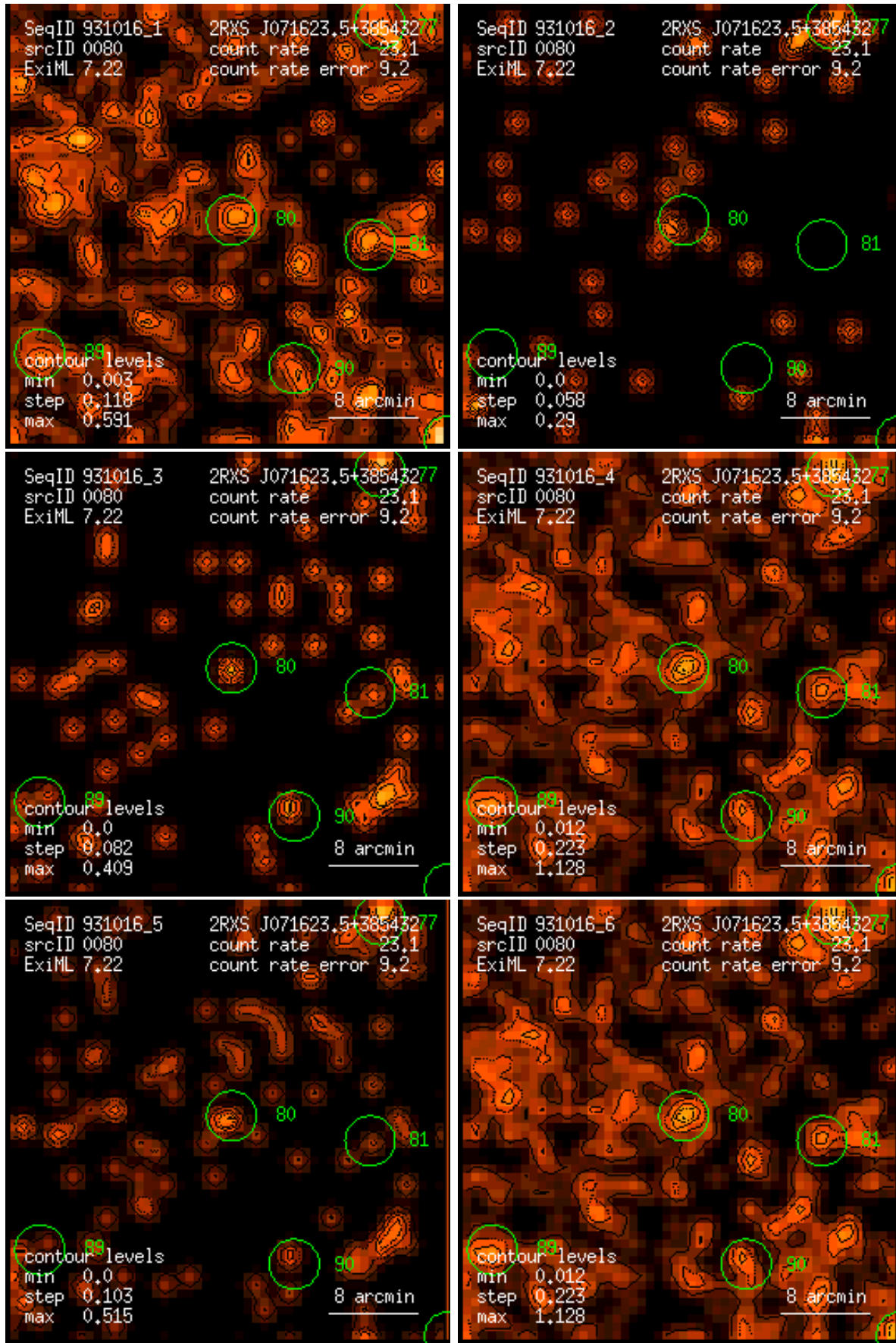
Figure 80: RASS 931016: detection 0080: band rate images, Gaussian filter: (1) PSPC channels 11 – 41, (2) 52 – 90, (3) 91 – 201, (4) 11 – 235, (5) 52 – 201, (6) 11 – 201. Broad band rates in counts/ks. Band rate contour levels in counts/ks/arcmin 2 .
