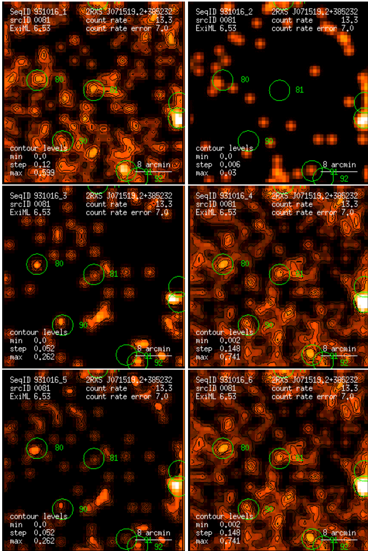
Figure 81: RASS 931016: detection 0081: band rate images, Gaussian filter: (1) PSPC channels 11 – 41, (2) 52 – 90, (3) 91 – 201, (4) 11 – 235, (5) 52 – 201, (6) 11 – 201. Broad band rates in counts/ks. Band rate contour levels in counts/ks/arcmin 2 .
