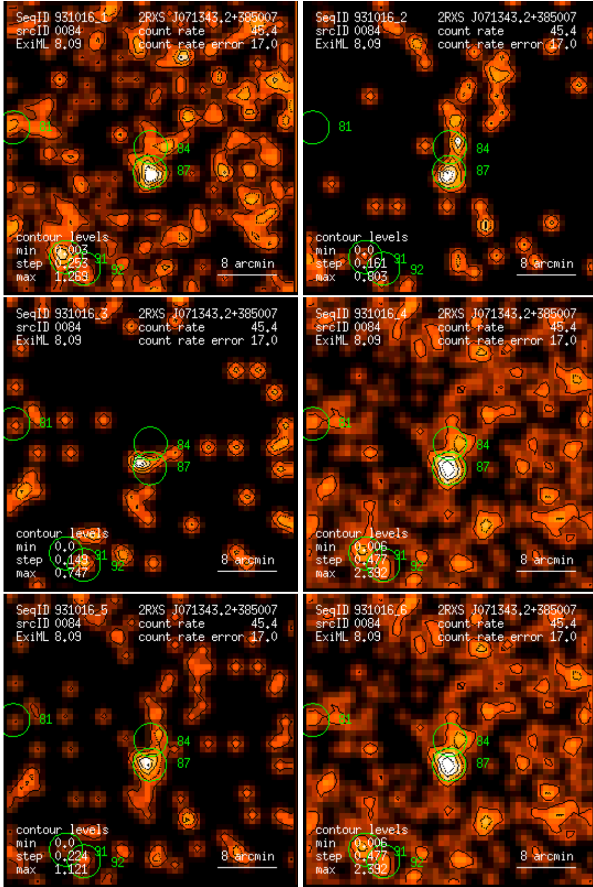
Figure 84: RASS 931016: detection 0084: band rate images, Gaussian filter: (1) PSPC channels 11 – 41, (2) 52 – 90, (3) 91 – 201, (4) 11 – 235, (5) 52 – 201, (6) 11 – 201. Broad band rates in counts/ks. Band rate contour levels in counts/ks/arcmin 2 .
