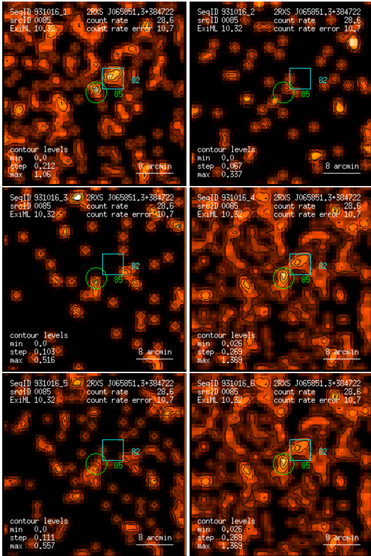
Figure 85: RASS 931016: detection 0085: band rate images, Gaussian filter: (1) PSPC channels 11 – 41, (2) 52 – 90, (3) 91 – 201, (4) 11 – 235, (5) 52 – 201, (6) 11 – 201. Broad band rates in counts/ks. Band rate contour levels in counts/ks/arcmin 2 .
