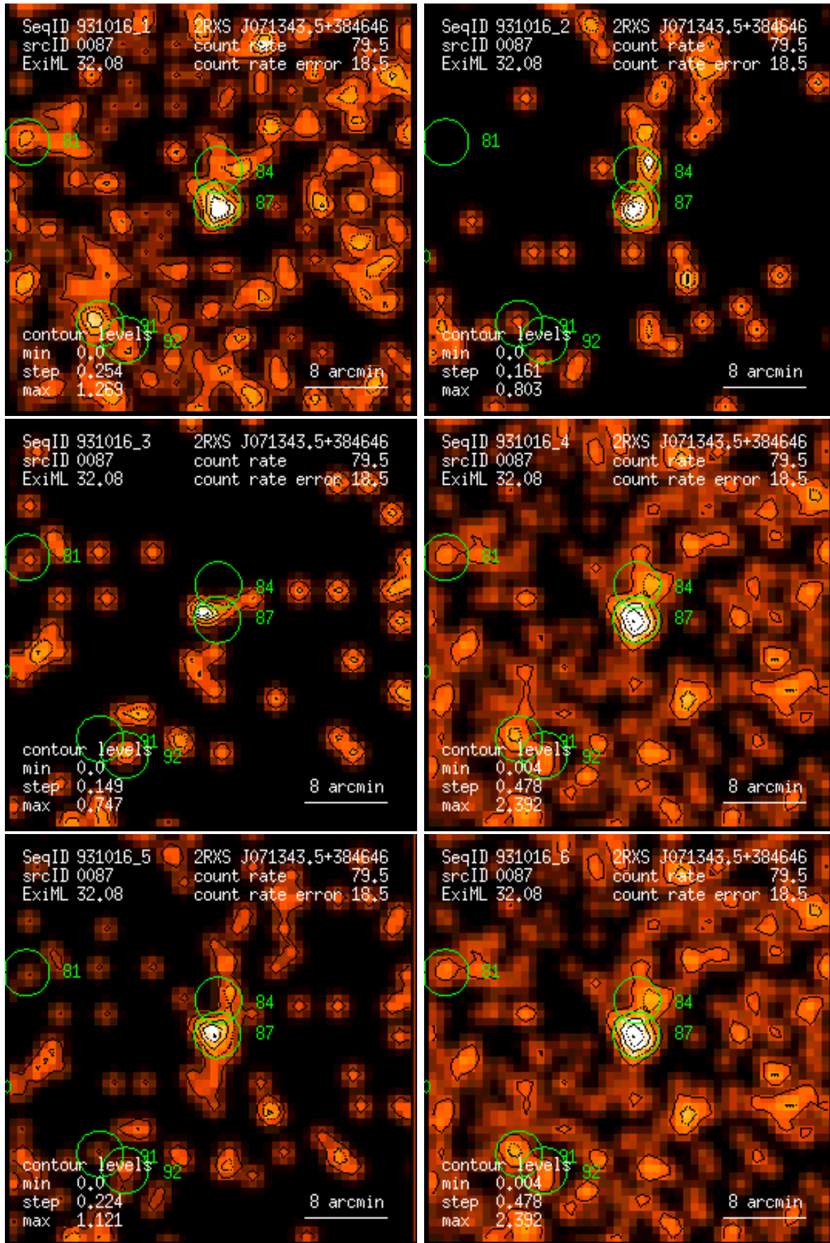
Figure 87: RASS 931016: detection 0087: band rate images, Gaussian filter: (1) PSPC channels 11 – 41, (2) 52 – 90, (3) 91 – 201, (4) 11 – 235, (5) 52 – 201, (6) 11 – 201. Broad band rates in counts/ks. Band rate contour levels in counts/ks/arcmin 2 .
